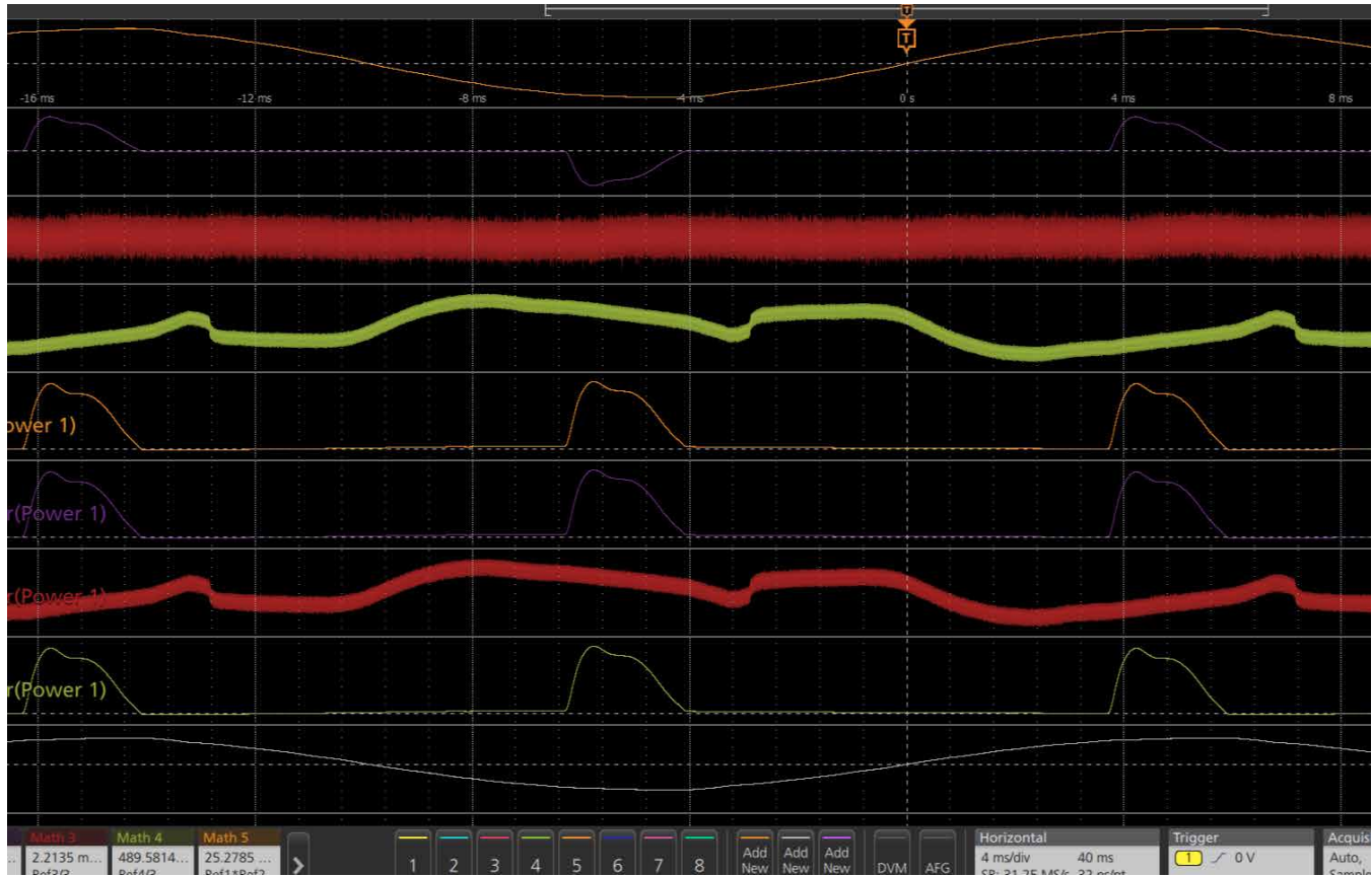
Efficiency measurement
