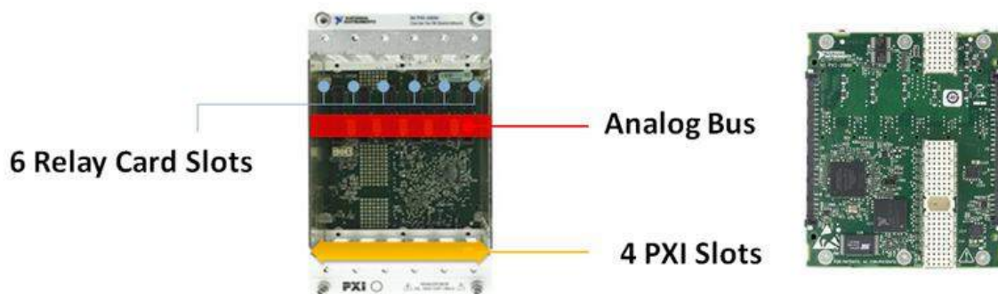
Figure 7. The PXI Carrier Module for SwitchBlock (PXI-2800) occupies four PXI slots, can hold up to six 1-slot Matrix Modules for SwitchBlock, and has an integrated analog bus designed to combine those matrix modules into a single large matrix, without additional external wiring.
