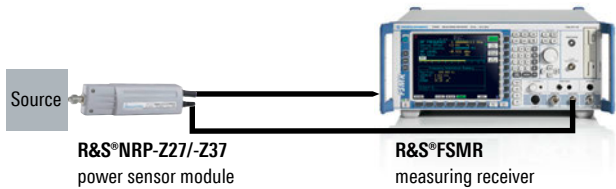
R&S®FSMR measuring receiver with R&S®NRP-Z27/-Z37 power sensor module
