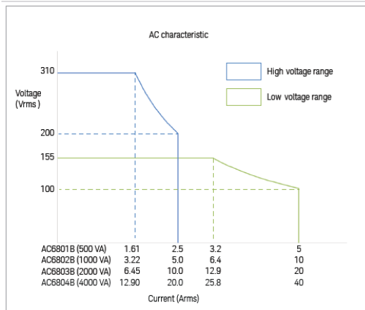
Figure 6. AC6800B steady-state AC output characteristic.
