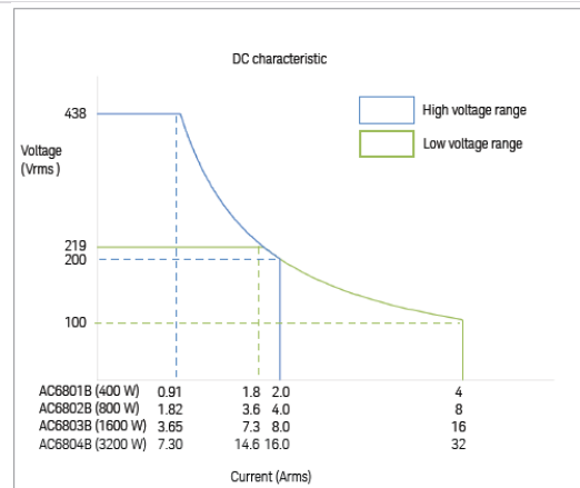
Figure 7. AC6800B steady-state DC output characteristics.
