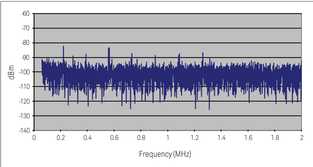
Figure 6. Keysight U1818A/B spurious versus frequency (typical)
