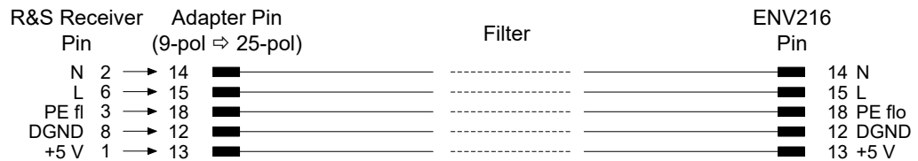
Figure 10-7: Connection from R&S ESRP to R&S ESH216
