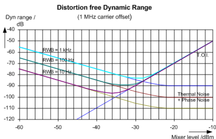
Figure 11-11: Intermodulation-free range of the R&S ESRP as a function of level at the input mixer and the set resolution bandwidth
