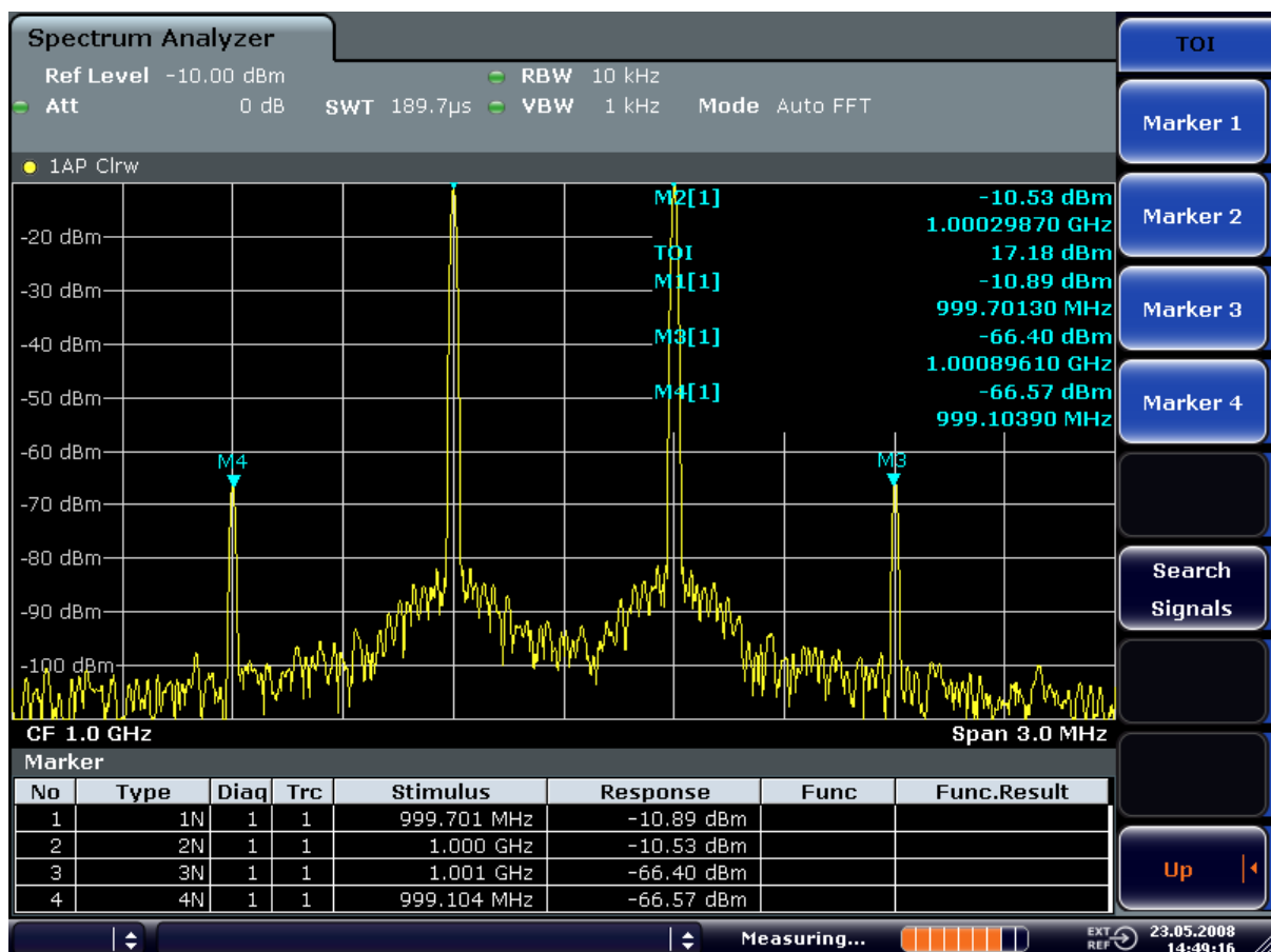
Figure 11-24: Result of intrinsic intermodulation measurement on the R&S ESRP.
