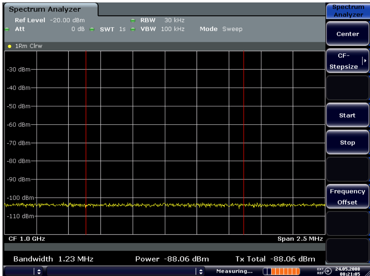
Figure 11-30: Measurement of the R&S ESRP's intrinsic noise power in a 1.23 MHz channel bandwidth.
