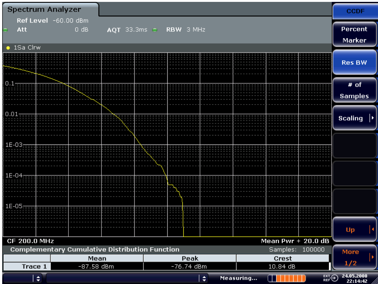
Figure 11-37: CCDF of white noise
