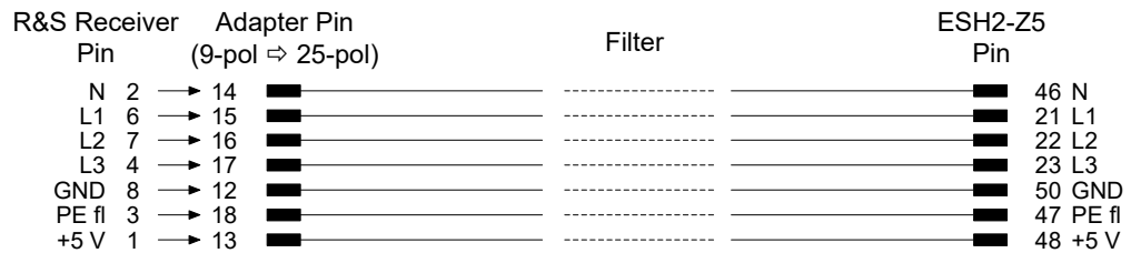
Figure 10-5: Connection from R&S ESRP to R&S ESH2-Z5
