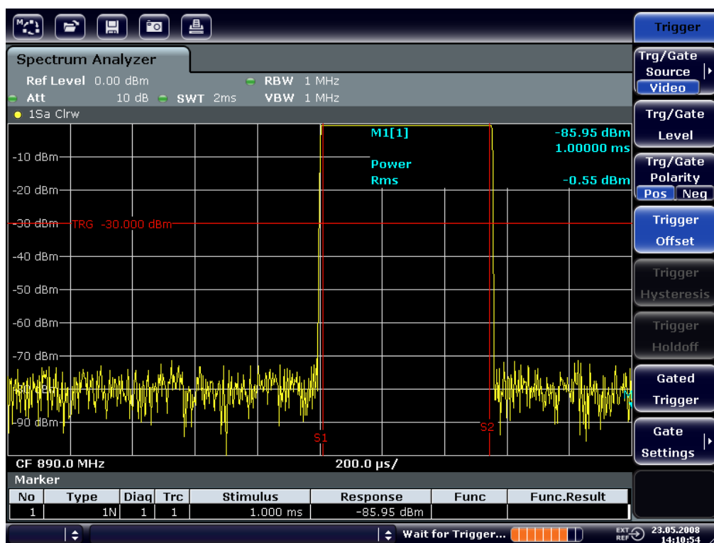
Figure 8-11: Power measurement during the activation phase of the burst
