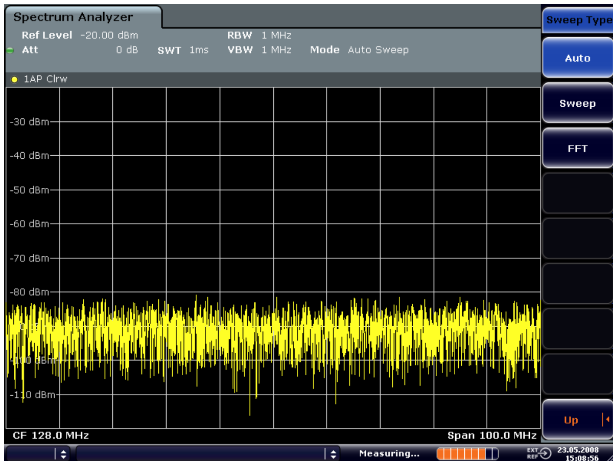
Figure 11-25: Sine wave signal with low S/N ratio. The signal is measured with the auto peak detector and is completely hidden in the intrinsic noise of the R&S ESRP.
