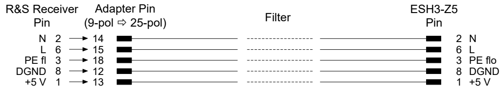
Figure 10-6: Connection from R&S ESRP to R&S ESH3-Z5
