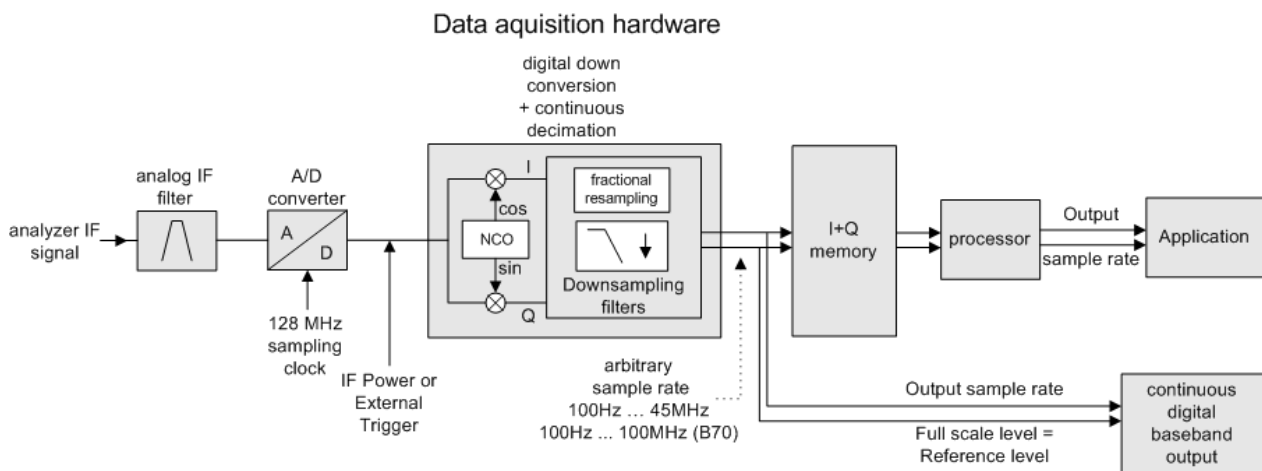
Figure 12-1: Block diagram illustrating the R&S ESRP signal processing
