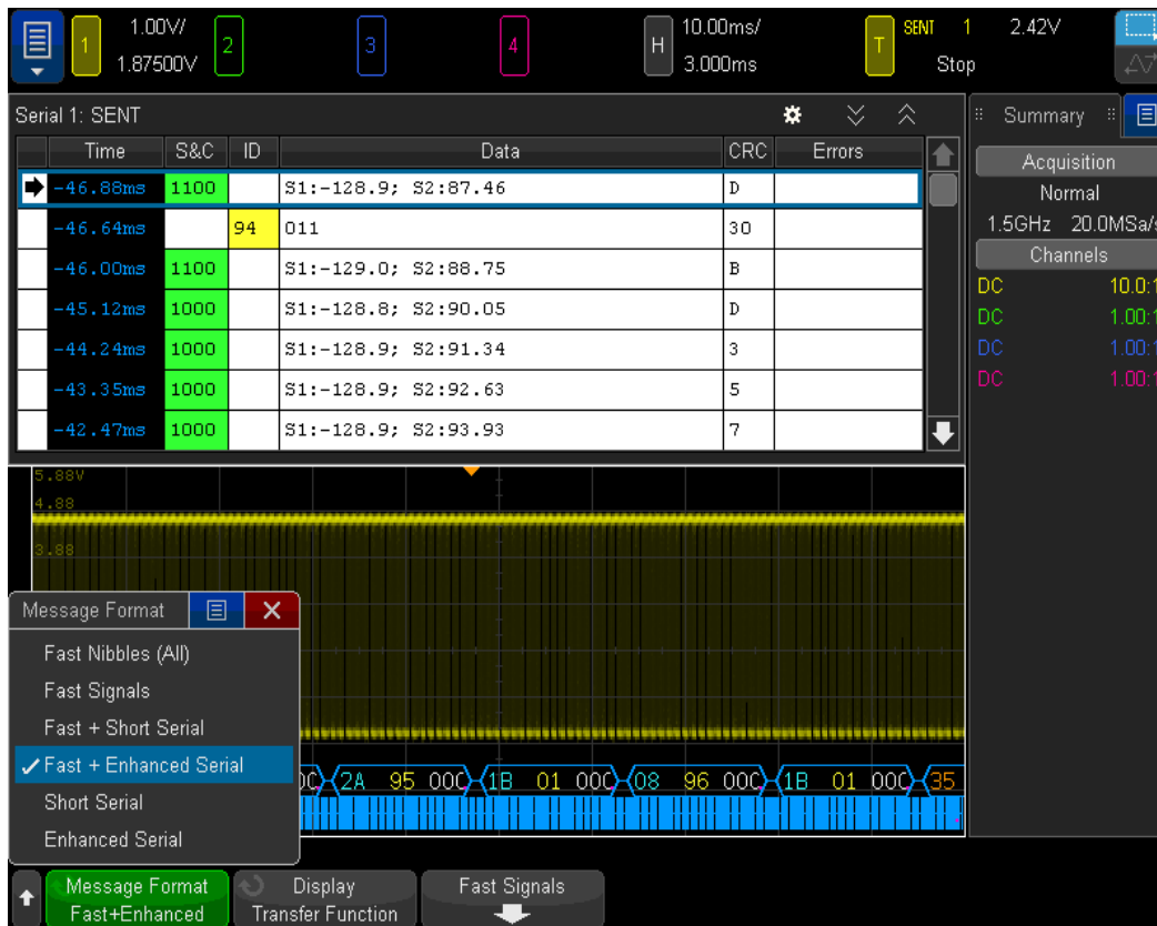
Figure 6. SENSE decode on an InfiniiVision X-Series oscilloscope.
