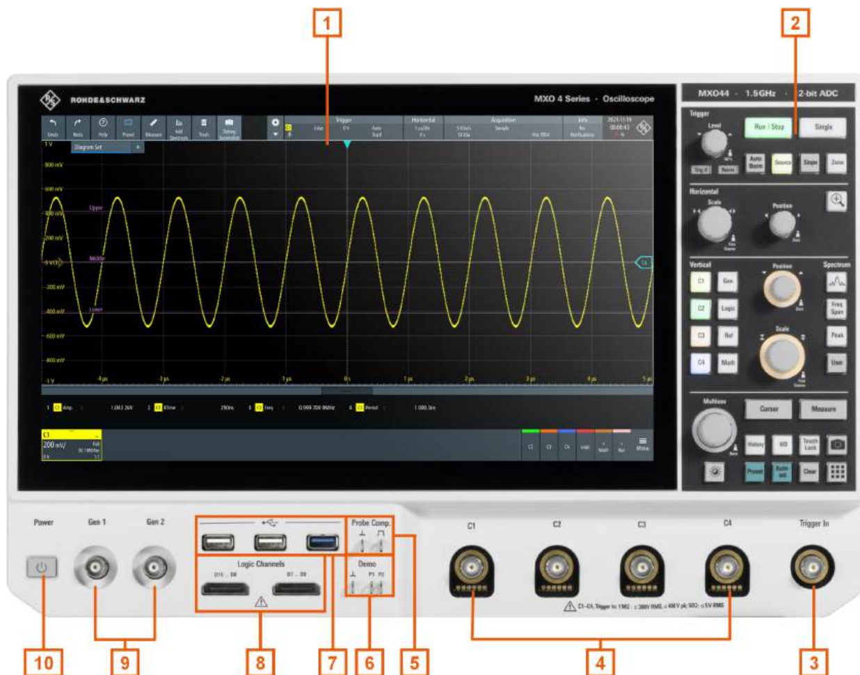
Figure 5-1: Front panel of MXO 4
