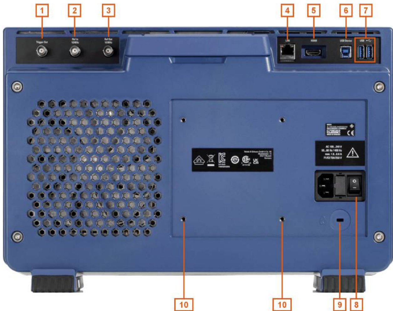
Figure 5-3: Rear panel view of MXO 4
