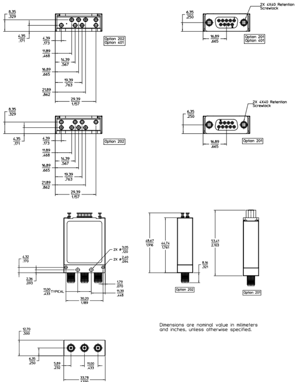
Figure 15. N1810UL dimension, SPDT, unterminated
