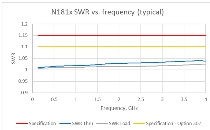
Figure 2. N181x (Option 004) return loss (SWR) vs frequency (GHz) typical
