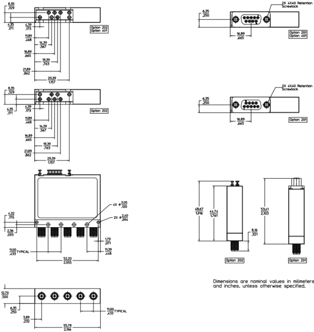
Figure 18. N1812UL dimension, 5-port bypass, unterminated
