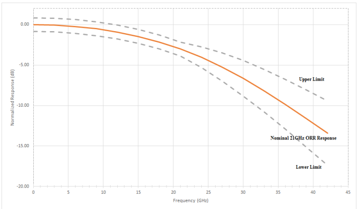
Fourth order Bessel-Thompson frequency response of the DPO70E1 Optical Probe and DPO7000SX ATI channel
