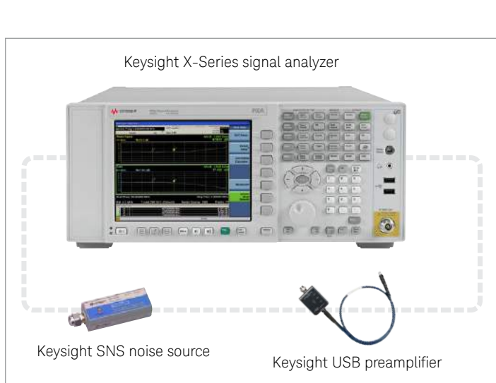
Figure 1. USB Preamplifier calibration setup
