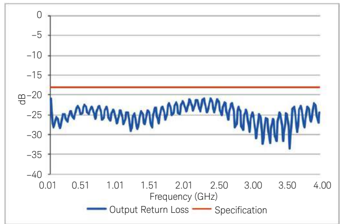
Figure 8. U7227/8A Output return loss versus frequency (typical)
