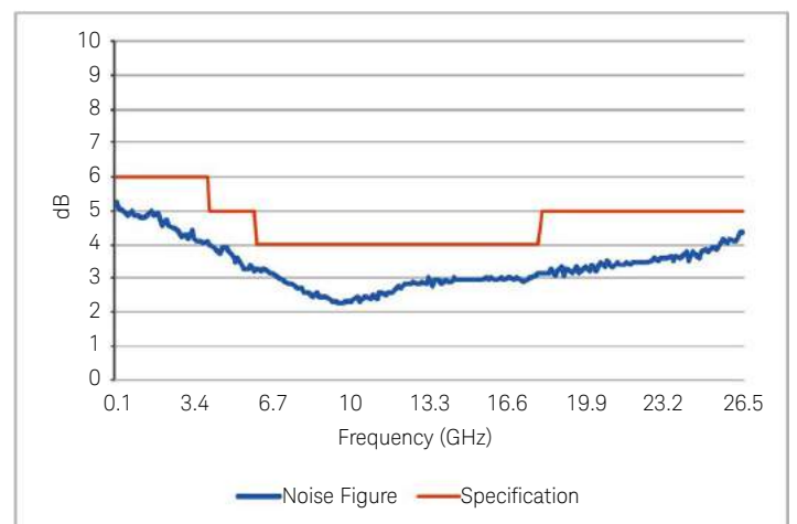
Figure 13. U7227/8C Noise figure versus frequency (typical)
