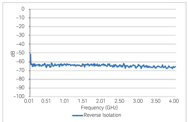
Figure 10. U7227/8A Reverse isolation versus frequency (typical)
