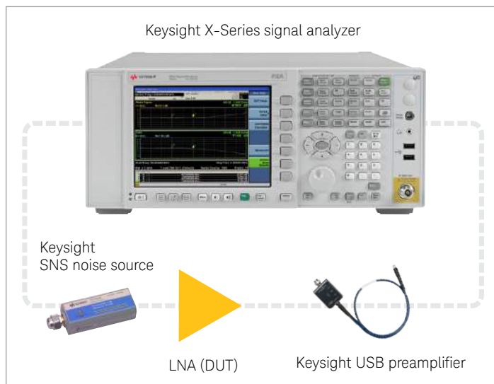
Figure 2. LNA noise figure measurement setup
