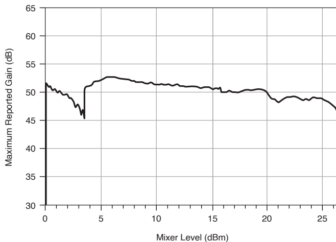
Figure 18. PXle-5606 Conversion Gain at 100 MHz BW
