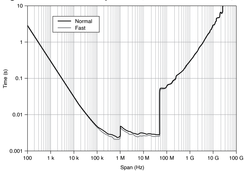
Figure 13. PXIe-5668 Analysis Time with 320 MHz and 765 MHz Bandwidth Setting for High Band
