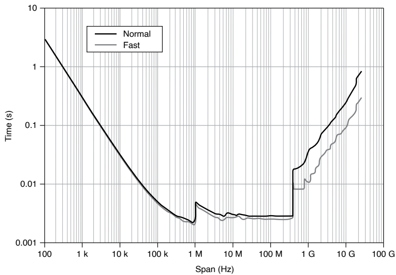
Figure 12. PXIe-5668 Analysis Time, Preselector Enabled (Nominal)
