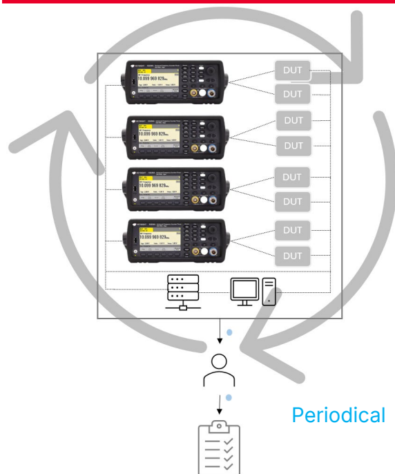
Automate Test Architecture 1 Test Station > 8 DUTs + 4 Counters
