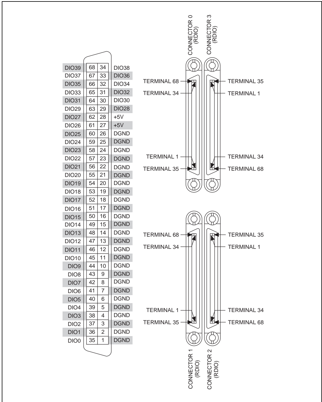
Figure 1. NI 781xR Connector Pin Assignments and Locations
