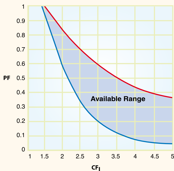
Figure 1: Crest Factor vs. Power Factor control Range
