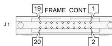
J1 Connector
