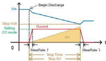
CC Mode
