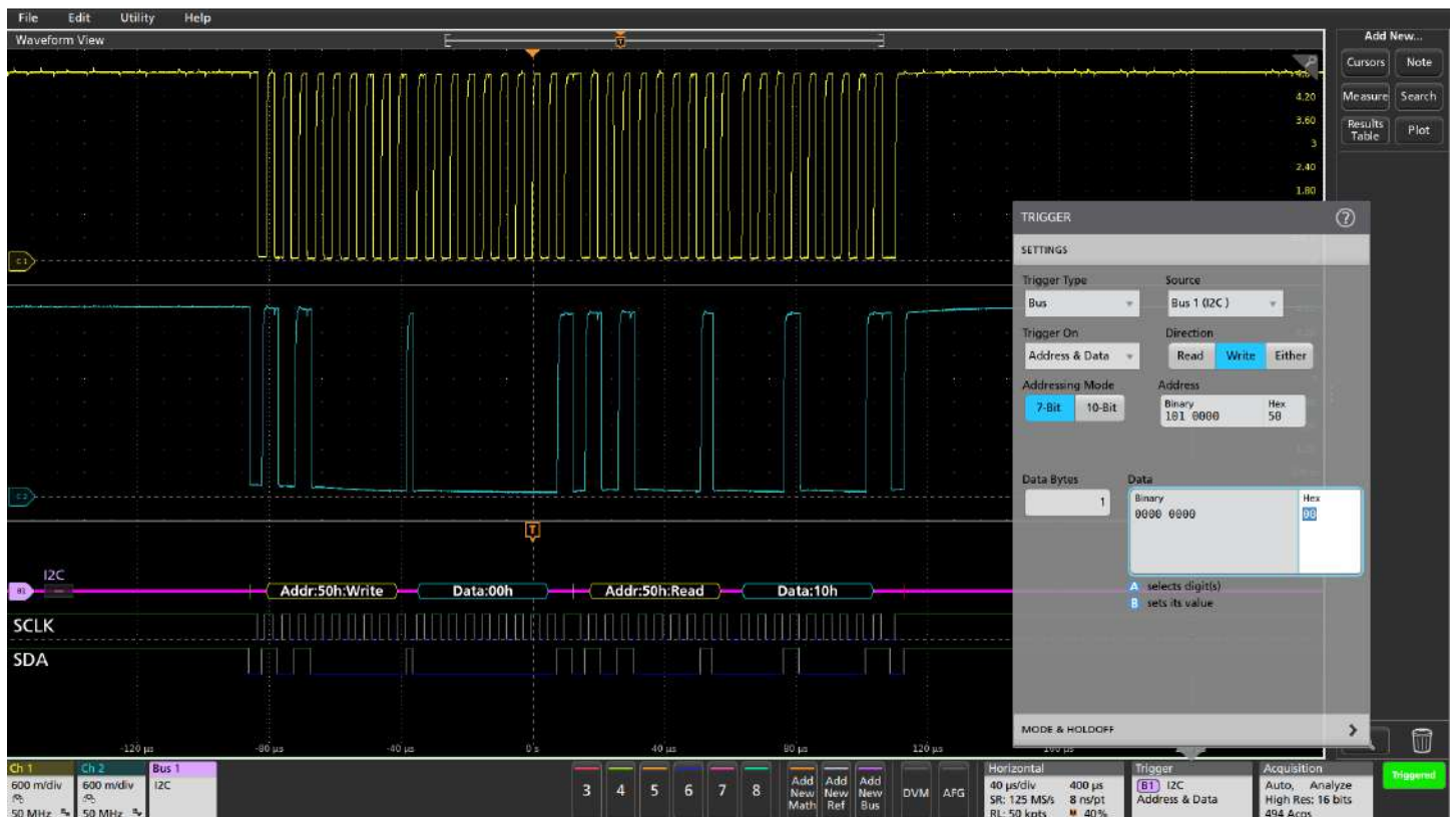
Triggering on a specific address value on the I2C bus.
