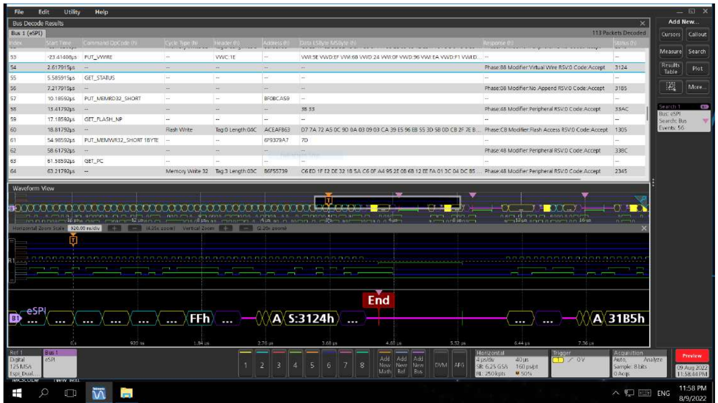
Searching on the Start/End event on the eSPI bus (Dual I/O Mode).
