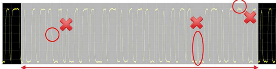
Figure 9. Another vendor's oscilloscope with 50,000 waveforms/second. A long dead time decreases your chances of capturing infrequent events.
