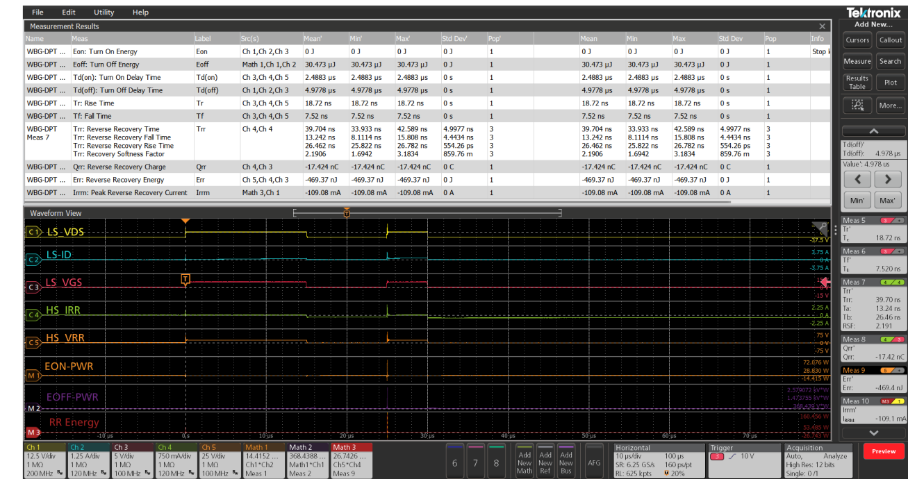
WBG-DPT measurements together, showing switching analysis, and timing parameters on the low side and diode reverse recovery measurements on the high side
