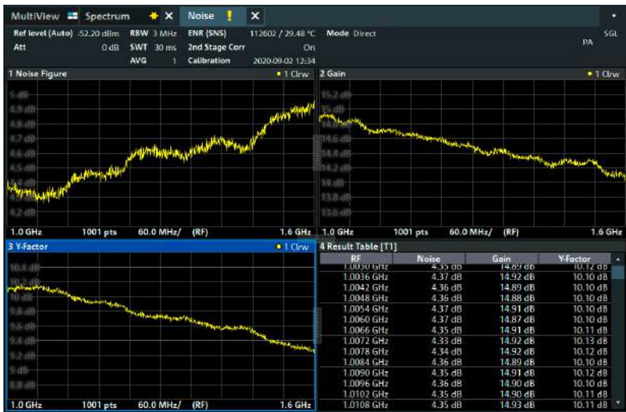
Simultaneous view of graphs for noise figure, gain and Y-factor versus frequency and a table of the results in numerical format
