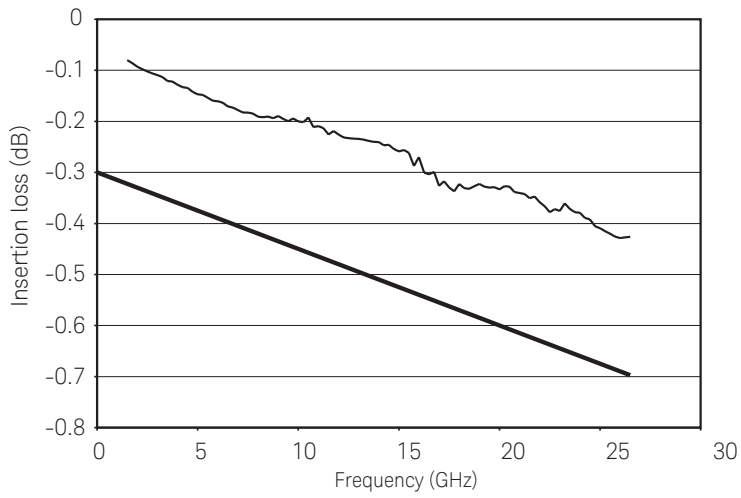
Figure 11. Keysight L-Series multiport switch insertion loss versus frequency
