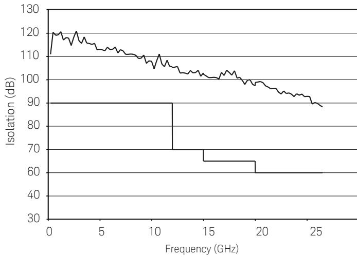
Figure 12. Keysight L-Series multiport switch isolation versus frequency
