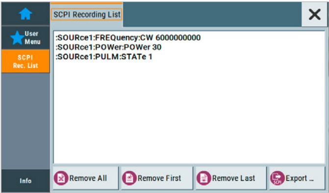
The built-in SCPI macro recorder and code generator supports fast, easy generation of SCPI program sequences.
