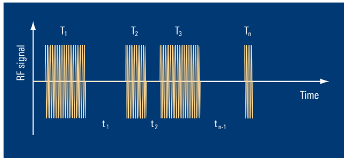
Pulse train
