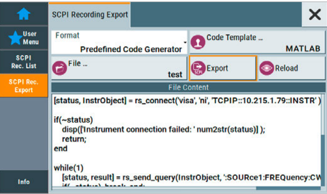
An SCPI program sequence generated with the built-in SCPI macro recorder.
