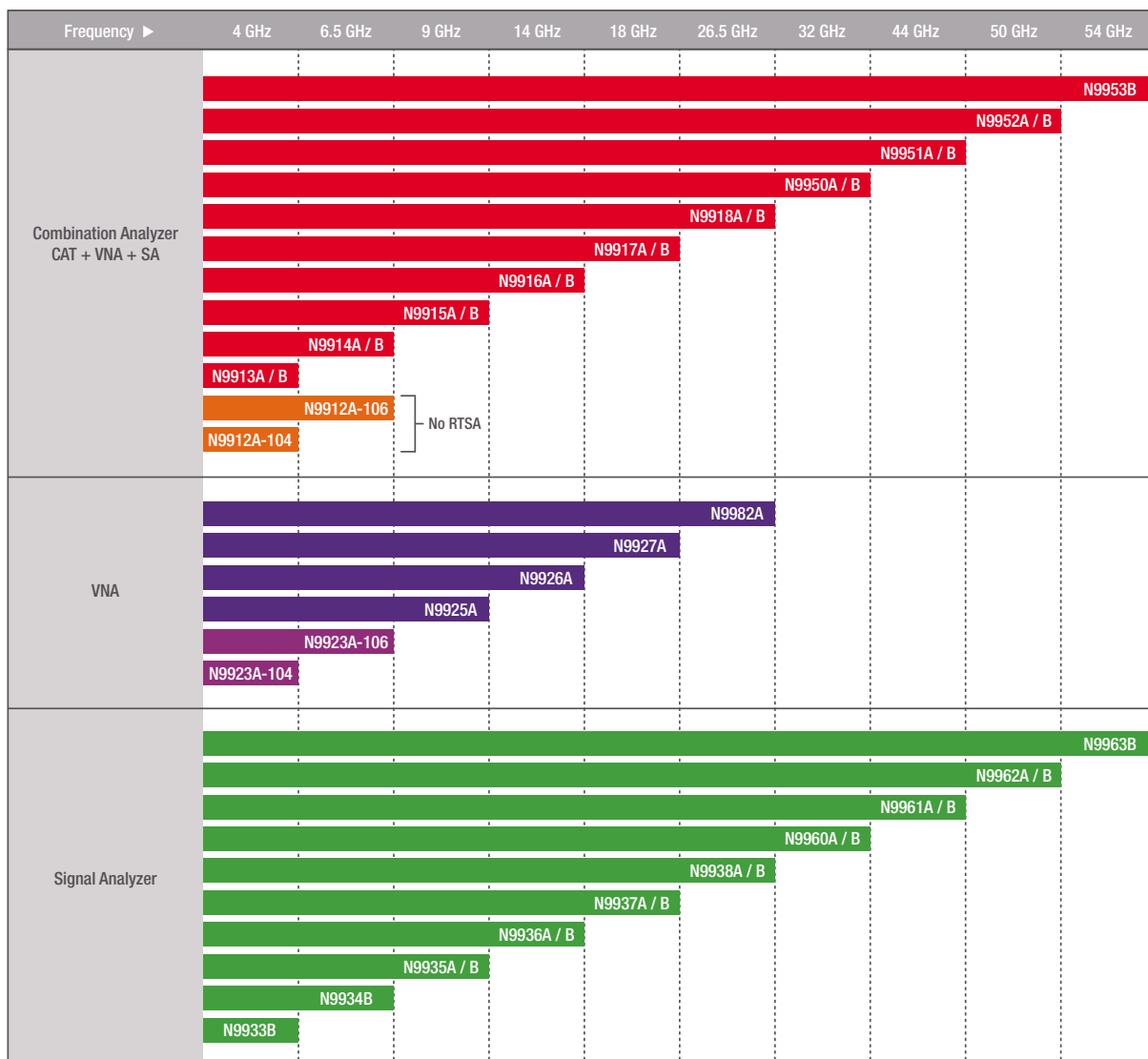
Figure 1. A visual representation of the FieldFox family, base configurations, and frequency coverage
