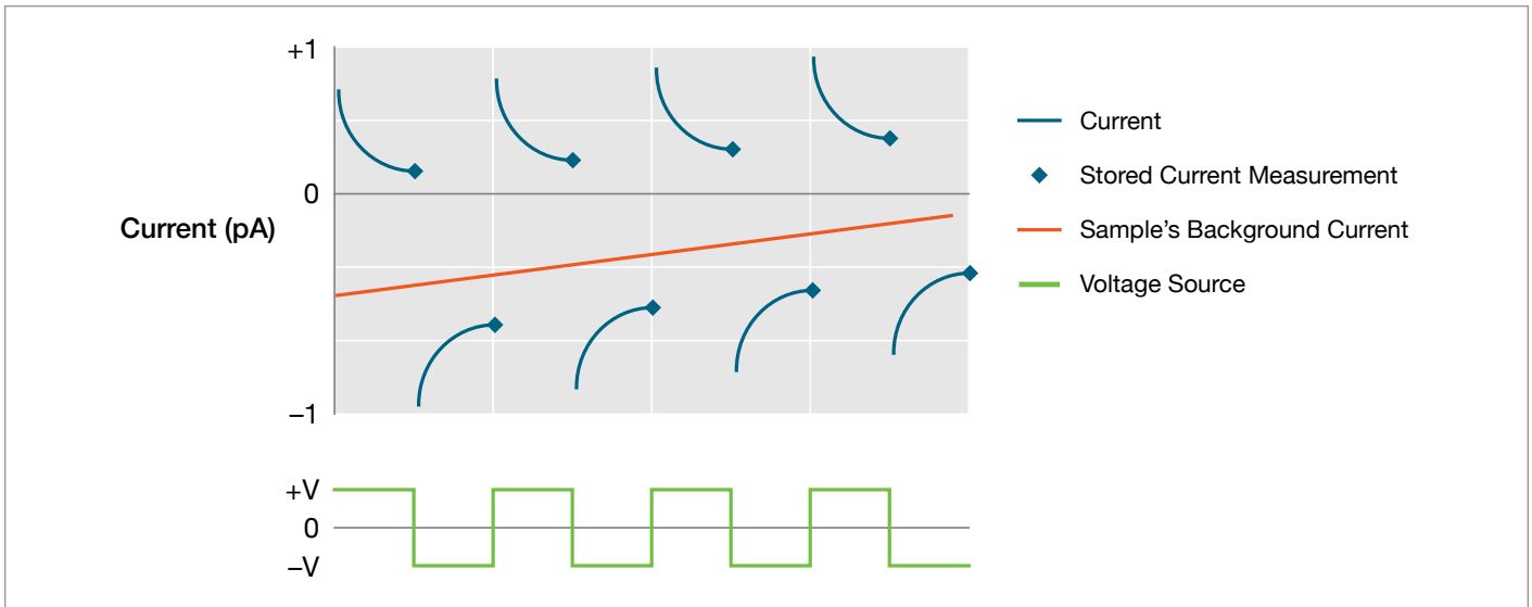
The alternating voltage source polarity method eliminates the effects of background currents in materials for making repeatable, accurate high resistance and resistivity measurements.
