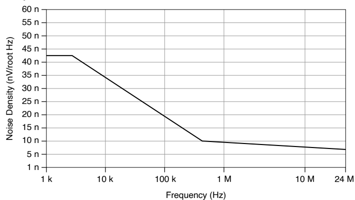
Figure 5. PXIe-5122 Spectral Noise Density, 0.2 V Input Range, Noise Filter Enabled, 1 M \Omega Input Impedance, Nominal
