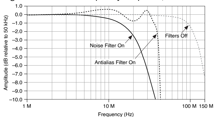
Figure 2. PXle-5122 Frequency Response, Measured
