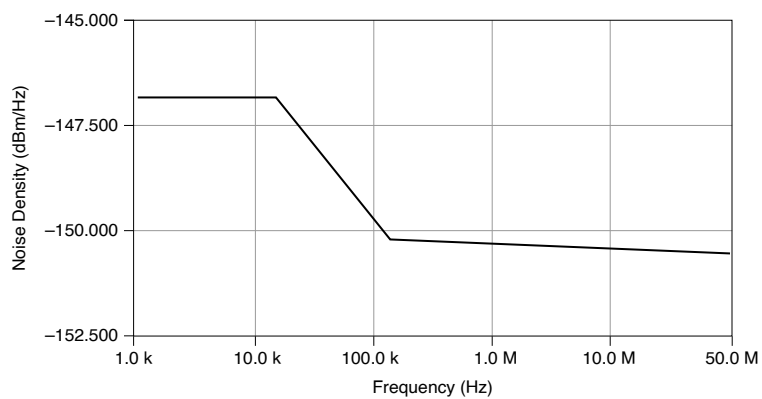
Figure 5. PXIe-5122 Spectral Noise Density, 0.2 V Input Range, Noise Filter Enabled, 1 M \Omega Input Impedance, Nominal
