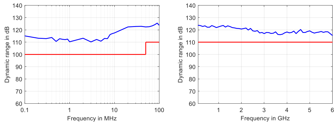
Measured dynamic range in dB versus frequency for the R&S®ZNLE3, R&S®ZNLE4 and R&S®ZNLE6
