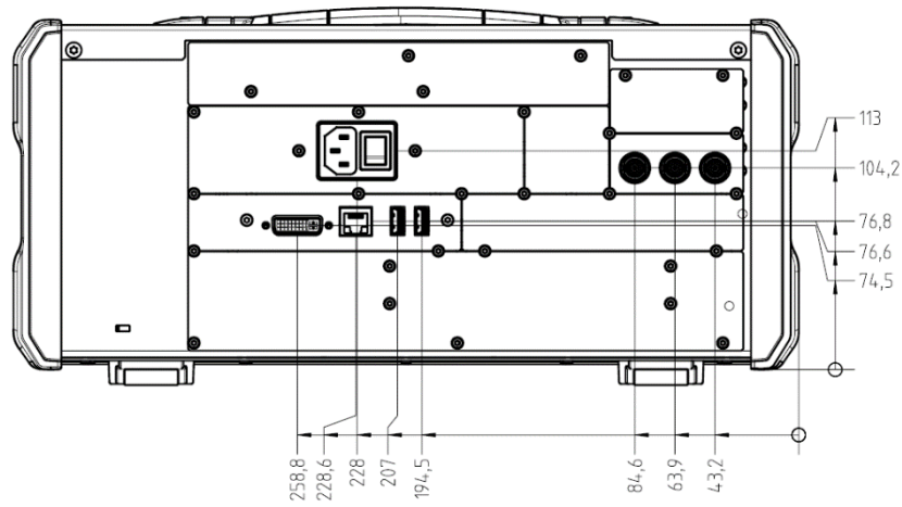
Rear view
