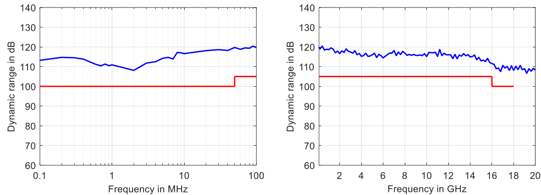
Measured dynamic range in dB versus frequency for the R&S®ZNLE14 and R&S®ZNLE18
