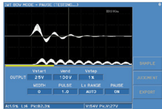
Figure 16 : Pause Function and Screenshot
