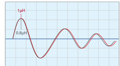
Figure 14 : With Compensation Voltage
