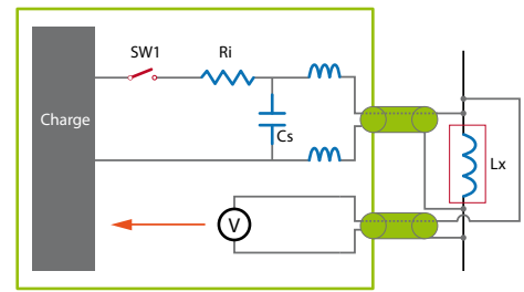
Figure 11 : 4-Terminal Measurement Diagram
