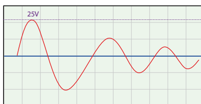
Figure 9 : Chroma 19301A Impulse Winding Tester
