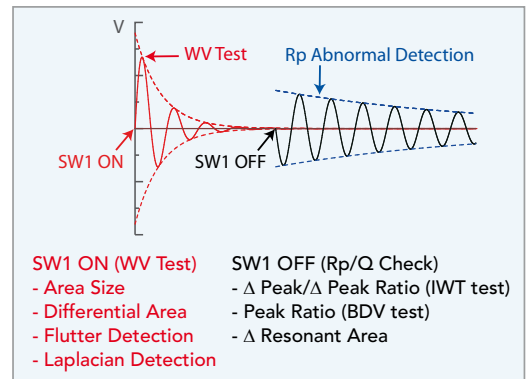
Figure 3: WW Test & Peak Ratio Waveform
