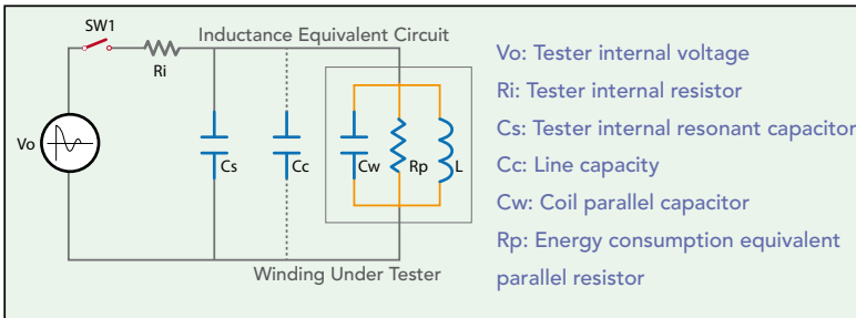
Figure 1: Equivalent Circuit
