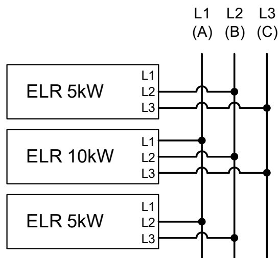
Figure 9 - Example for AC wiring of multiple units with different power ratings and almost balanced current
