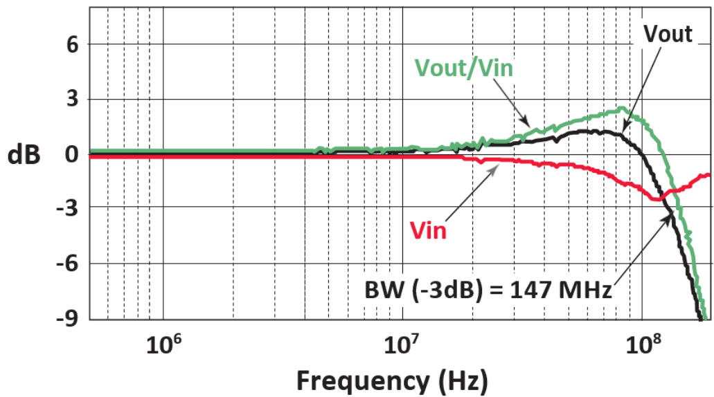
Figure 4. V_{out}/V_{in} vs. frequency response of N2790A.
