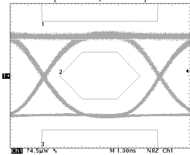
OC-3/STM-1 SONET/SDH Transmitter Eye Pattern Test.
