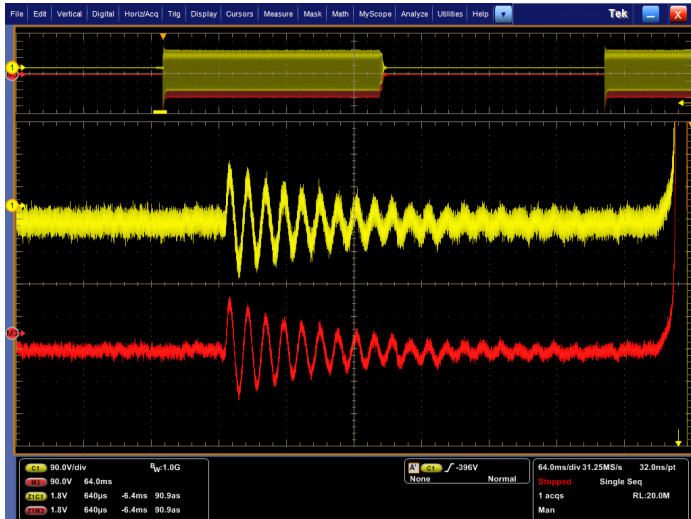
Capture - HiRes acquisition - increased vertical resolution to >11 bits while removing noise on a 650 V Pk-Pk signal while seeing the smaller details of less than 1 V Pk-Pk with or without apply low-pass filtering.
