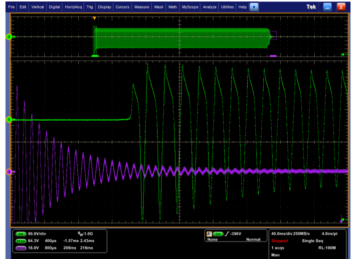
Capture - 100 Meg point acquisition with HiRes acquisition - increase vertical resolution to >11 bits with dual zoom of waveform details.
