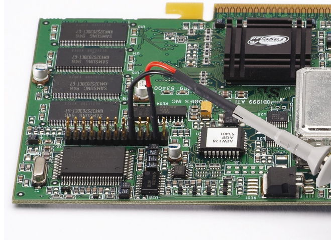
Figure 7. The dual lead adapter allows you to easily connect the N2870A Series probe to a popular 0.1" pin header with 0.025" square pins. This dual lead adapter has no shorting hazards since all external metal surfaces are insulated.
