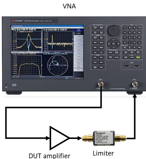
Figure 1. Typical application
