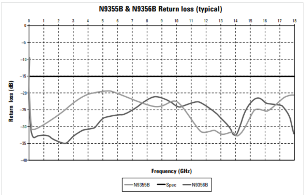
Figure 6. N9355/6B typical return loss versus frequency
