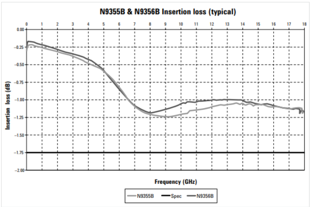
Figure 5. N9355/6B typical insertion loss versus frequency
