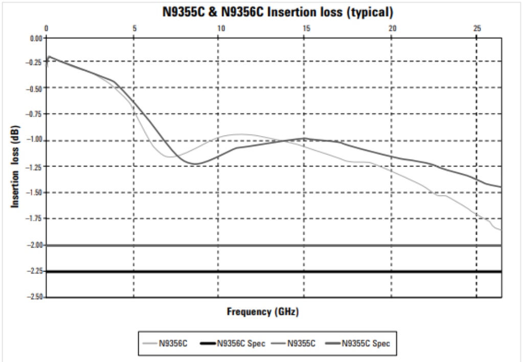
Figure 7. N9355/6C typical insertion loss versus frequency
