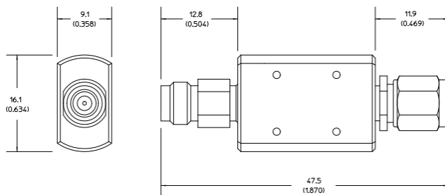
Figure 15. N9355F mechanical dimension
