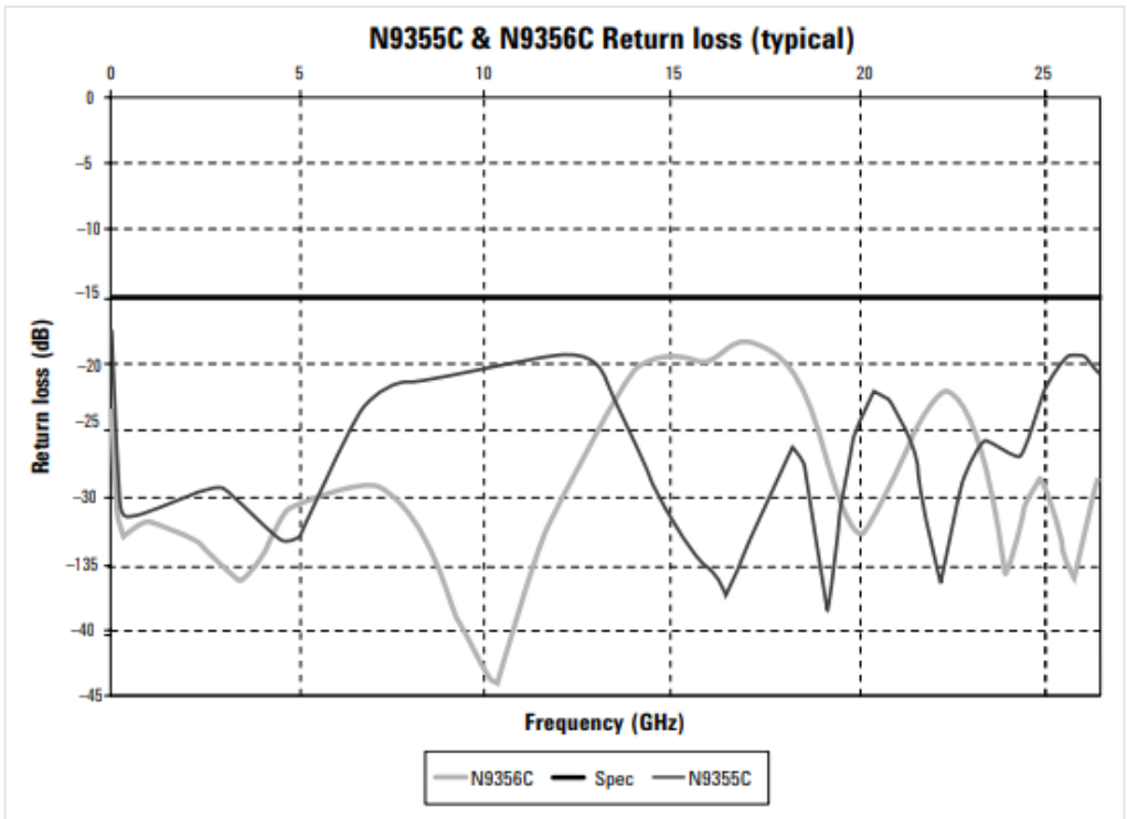
Figure 8. N9355/6C typical return loss versus frequency
