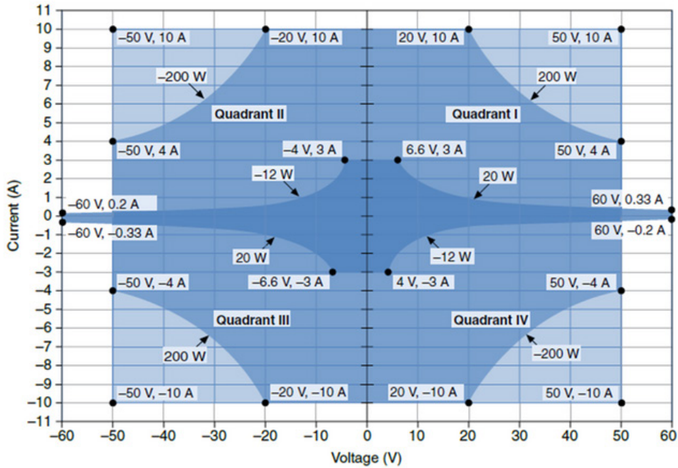
FIGURE 7 The PXIe-4139 can generate pulses up to 10 A with lengths between 50 \mu s and 1 ms.
