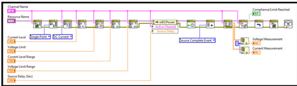
FIGURE 8 LabVIEW VI using the DC-Power API
