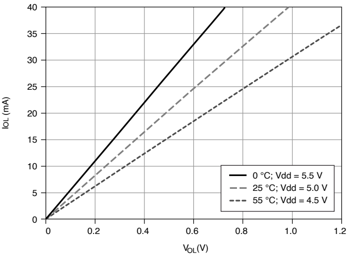
Figure 10. P0.<0..7>: I OL versus V OL
