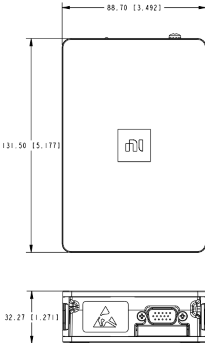
Figure 1. cDAQ-9170 Dimensions
