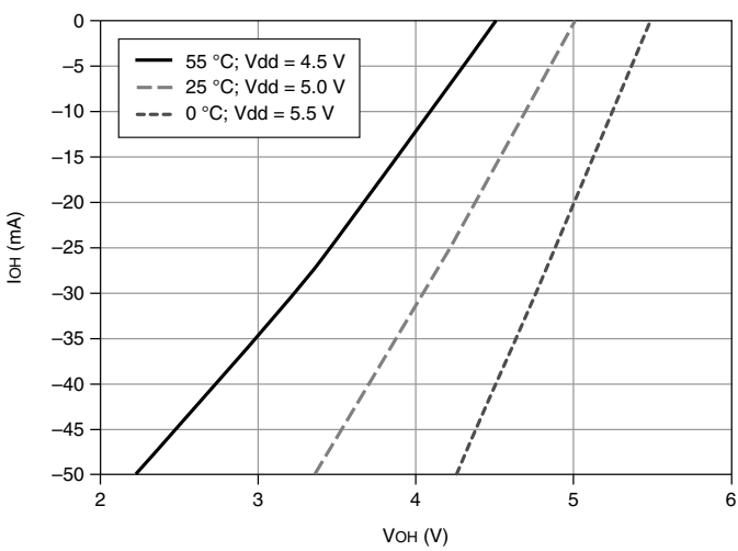
Figure 3 : P0.<0..7>: I OH versus V OH
