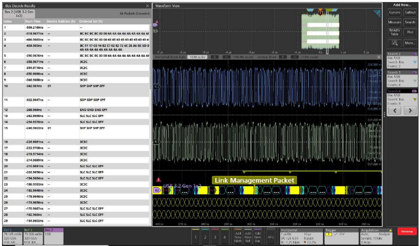
USB bus setup and MixedHex display, showing decode with speed USB 3.2 Gen 1x2 with the results table on left of the graticule, search on packet type LMP along with lane 0 and lane 1 search on training sequence is added.
