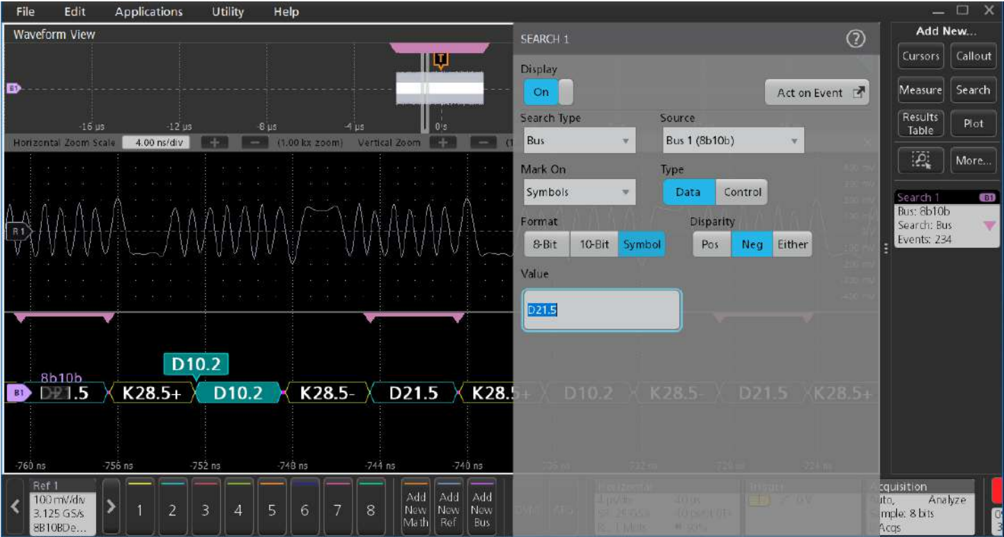
Searching on a specific data symbol in symbol format on a 8B10B bus.
