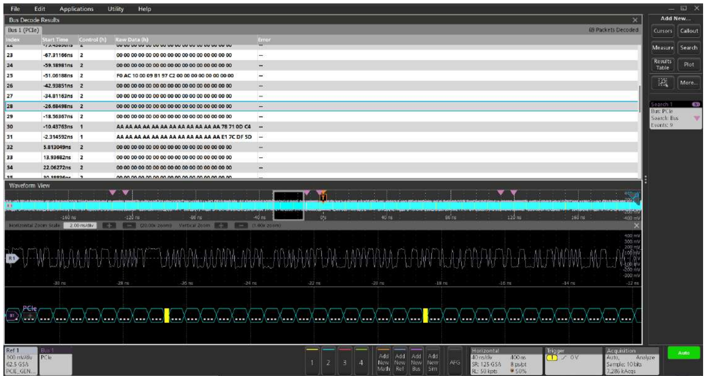
PCIe Gen4 bus setup showing decode with packet view Off.
