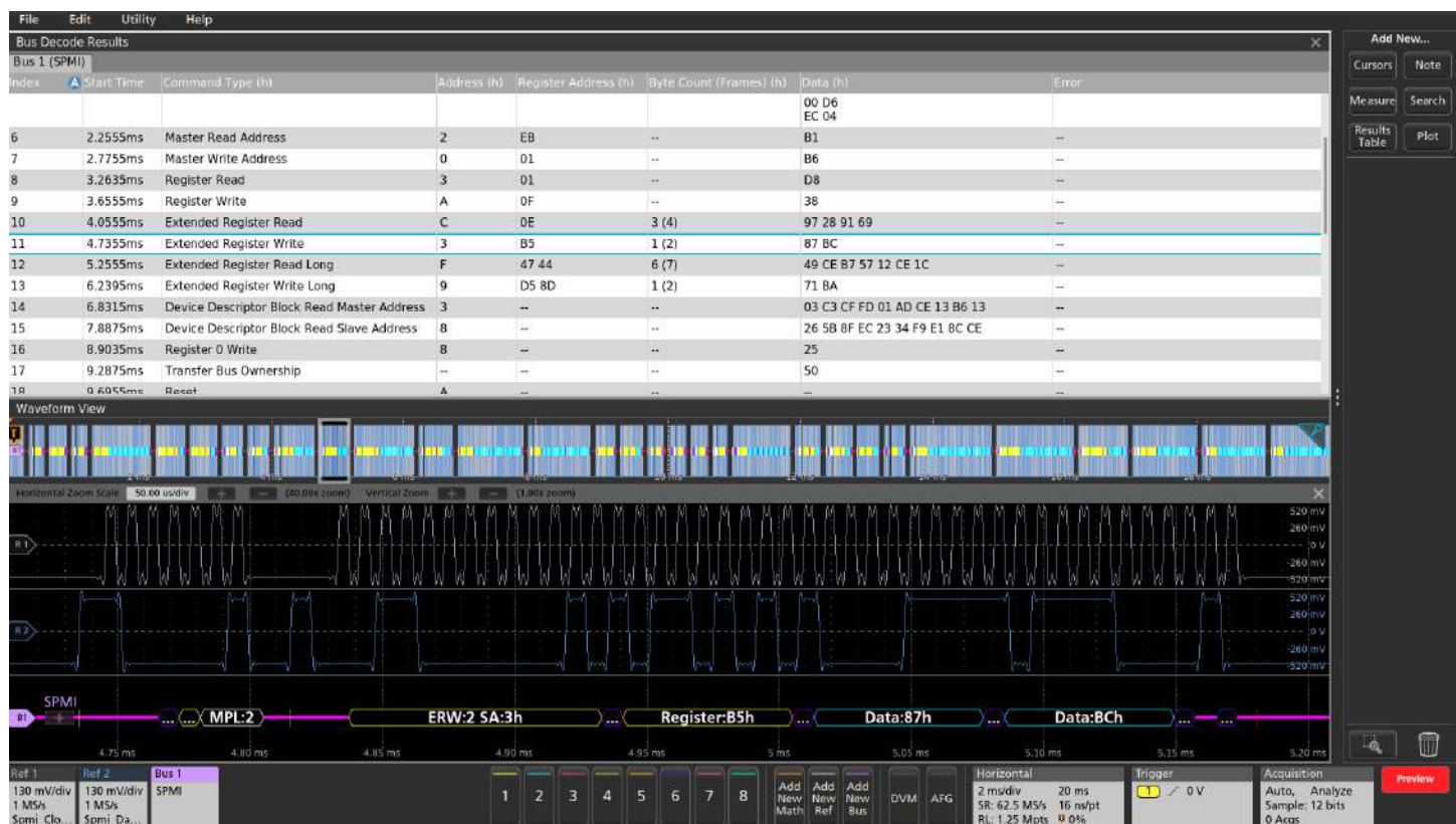
Protocol Decode Results Table provides a time-stamped, tabular view of all captured packets on the SPI bus.
