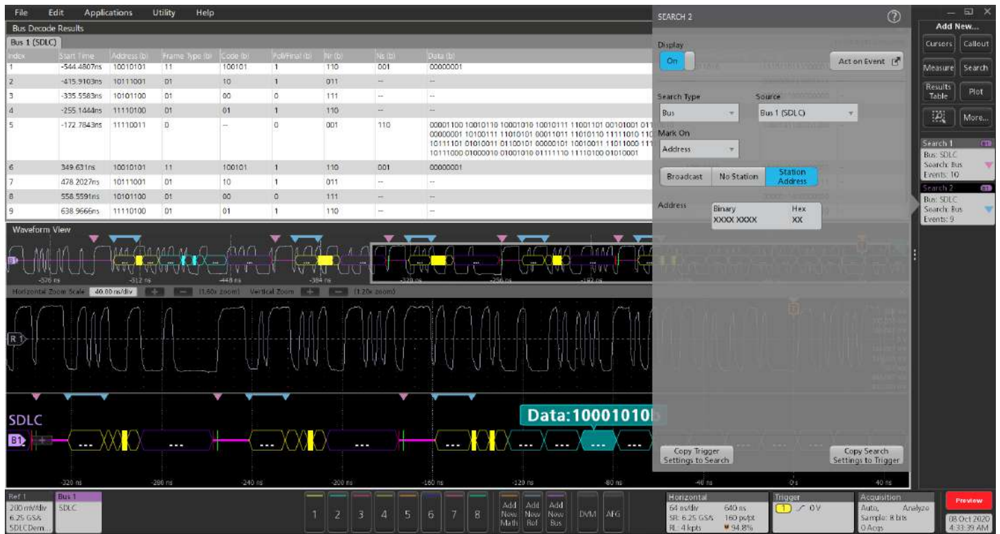
Searching on a station address on the SDLC bus.
