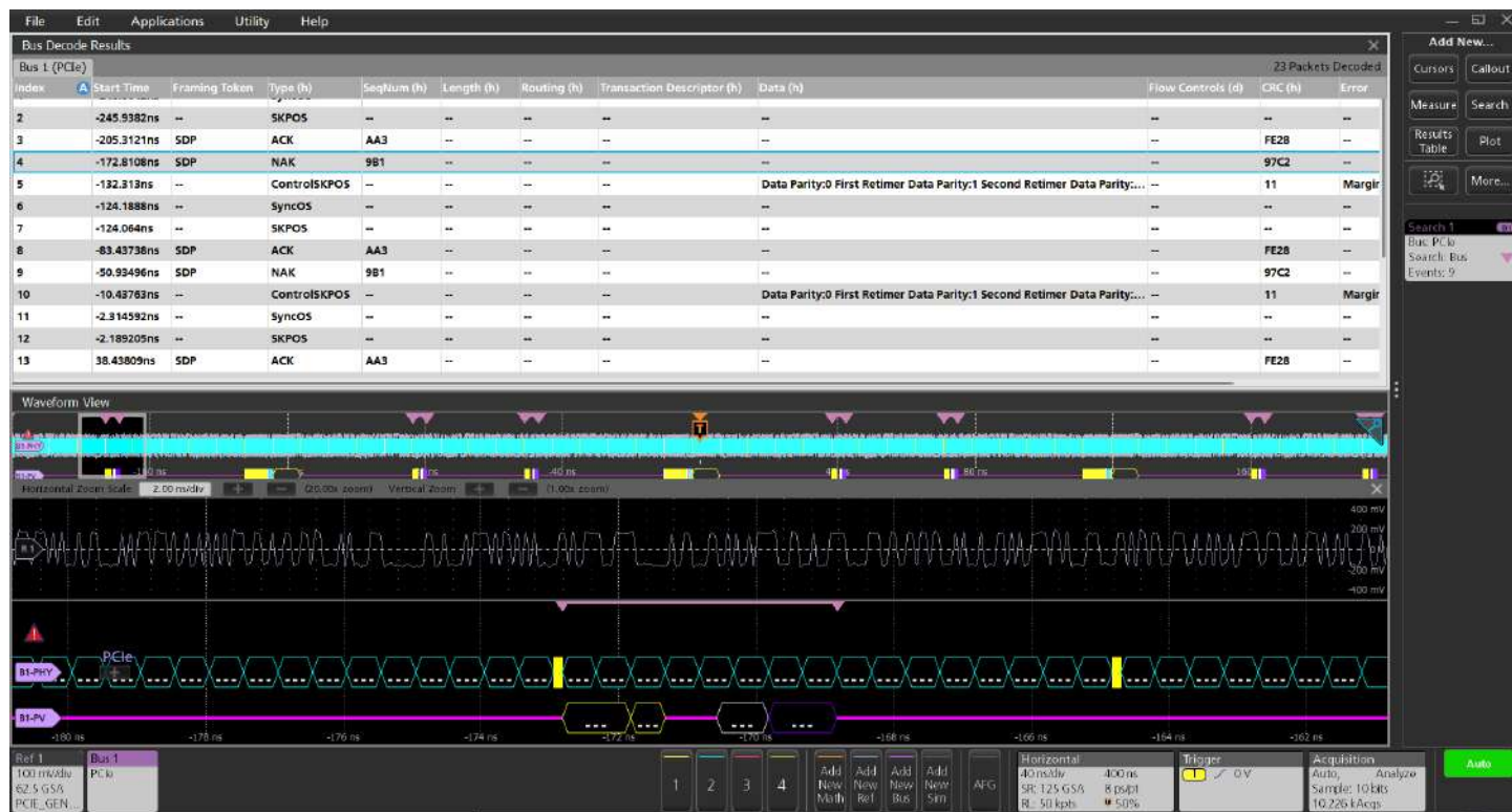
PCIe Gen4 bus showing decode with packet view On. DLP packet of type ACK was searched with 9 occurrences.
