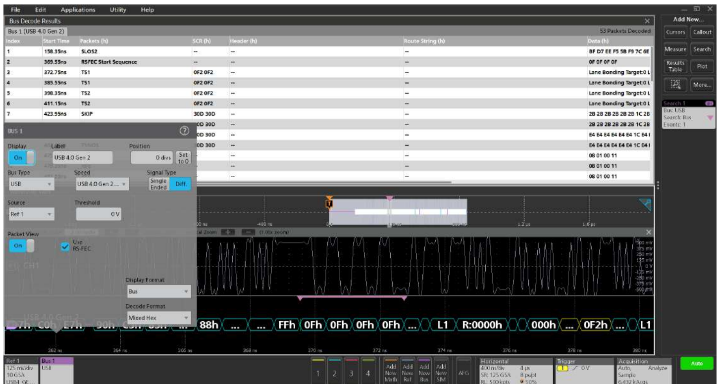
USB4 Gen2 bus setup showing decode with packet view ON with RSFEC. START_RSFEC searched with 1 occurrence.
