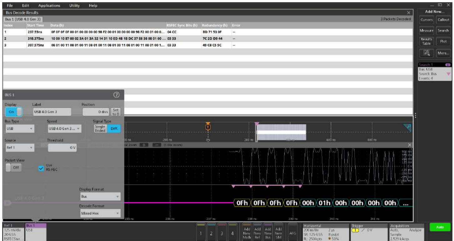
USB4 Gen3 bus setup showing decode with packet view Off with RSFEC. START_RSFECSearched with 4 occurrences.
