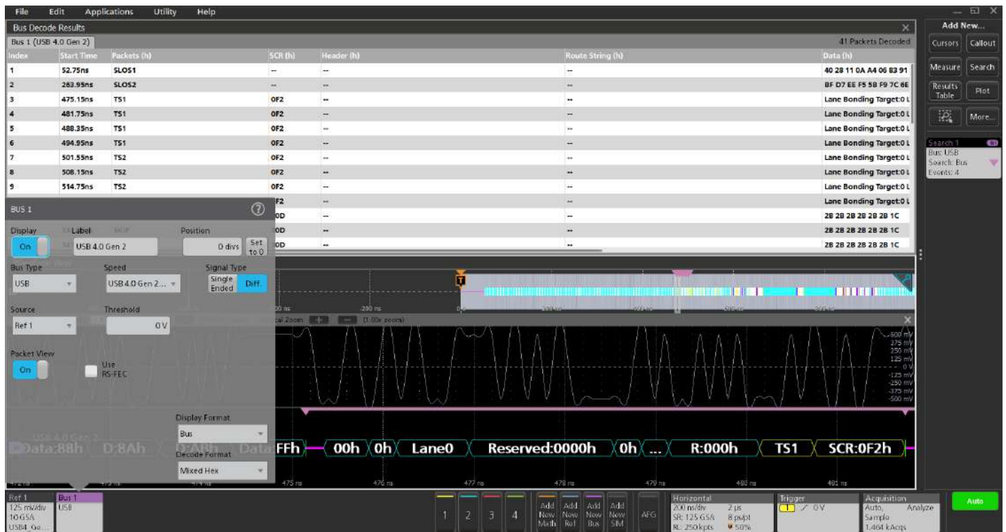
USB4 Gen2 bus showing decode with packet view ON. Ordered Set of type TS1 was searched with 4 occurrences.
