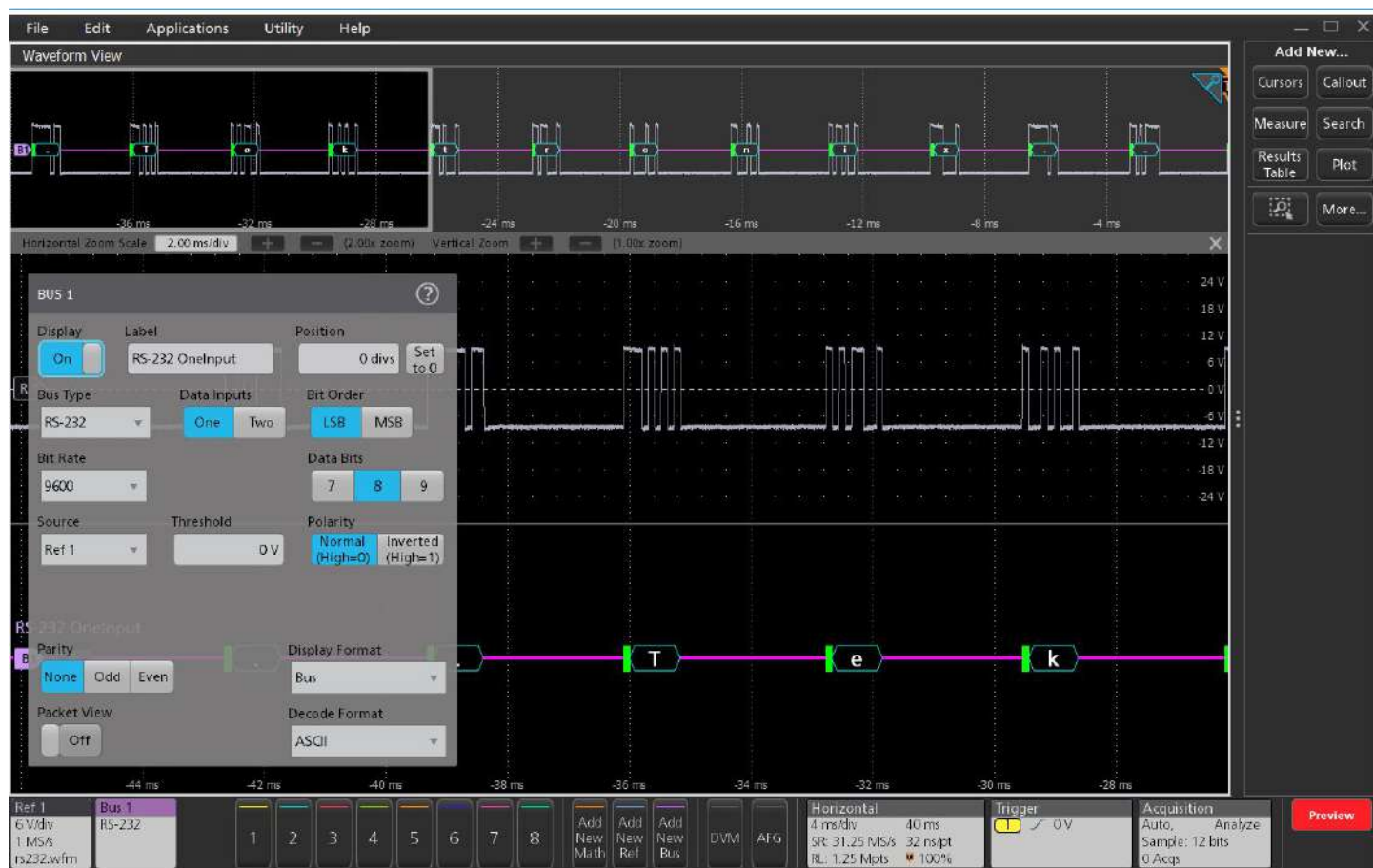
RS-232 bus setup and ASCII display, showing assignment of source signal, digital threshold, and polarity.
