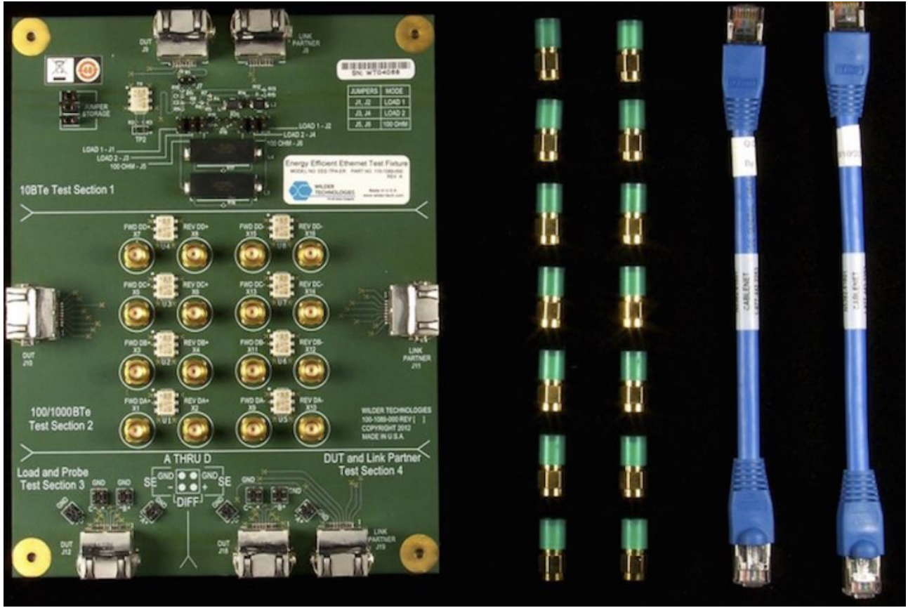
Figure 9. The EEE-TPA-ERK Wilder Technologies Energy Efficient Ethernet test fixture allows you to test to the 10BASE-T e , 100BASE-T Xe and 1000BASE-T e Energy Efficient Ethernet standards. Sold separately through Wilder-Technologies.
