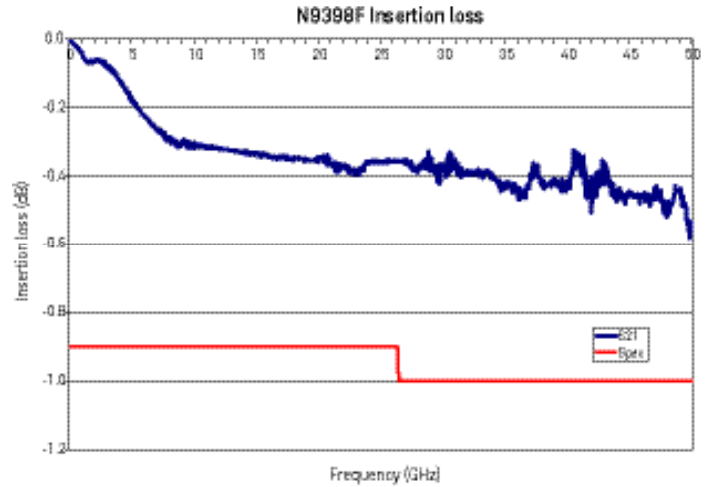
Figure 11. N9398F typical insertion loss versus frequency
