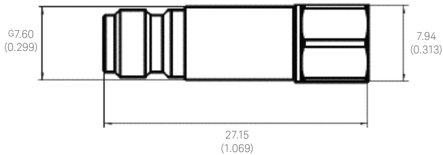
Figure 4. N9398/99F product outline
