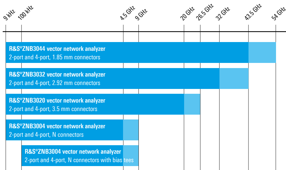
R&S®ZNB3000 models
