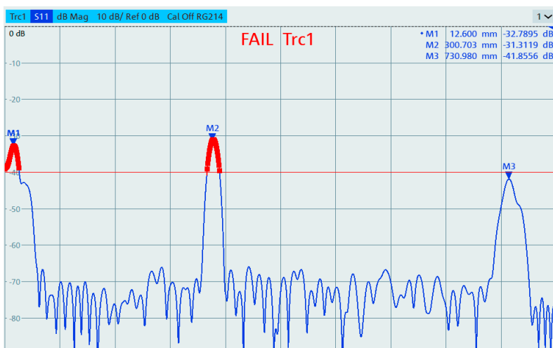
Reflections on a cable terminated with 40 dB:
