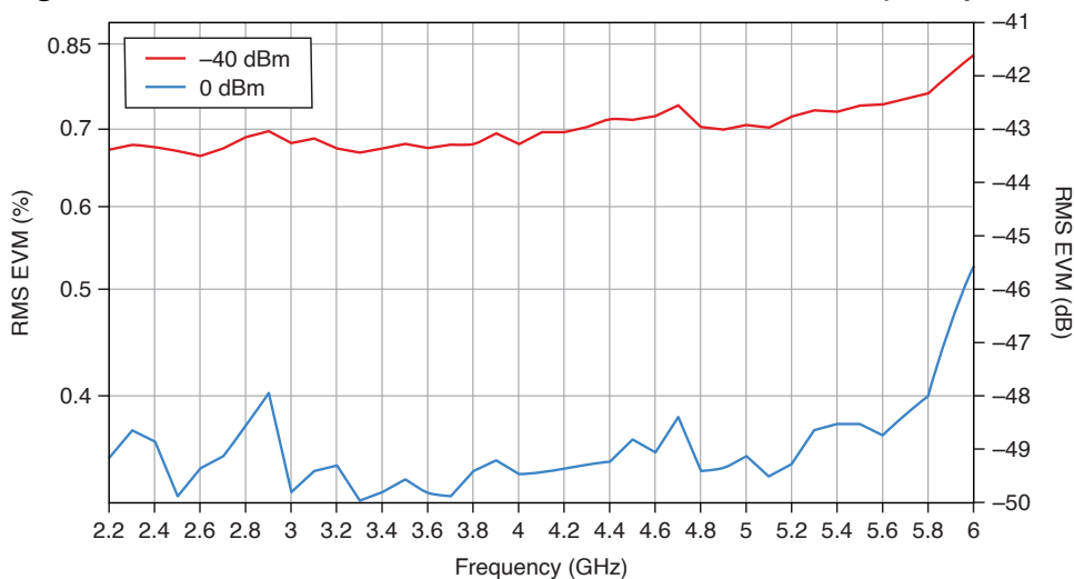
Figure 23. 5G NR Measured RMS EVM (dB and %) Versus Frequency (Hz)
