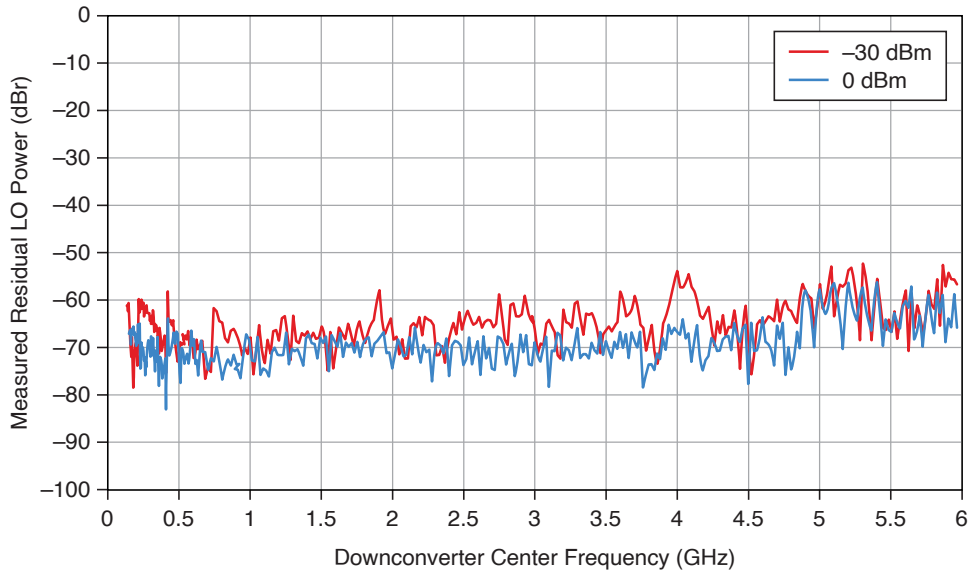
Figure 9. Input LO Residual Power, Measured (PXIe-5841 with PXIe-5655)
