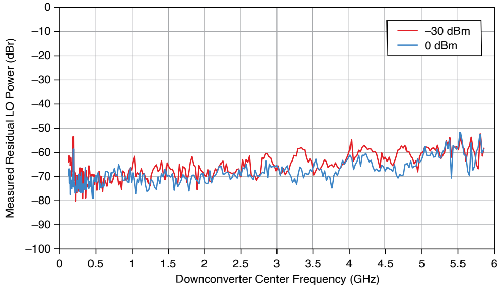
Figure 9. Input LO Residual Power, Measured (PXIe-5841 with PXIe-5655)
