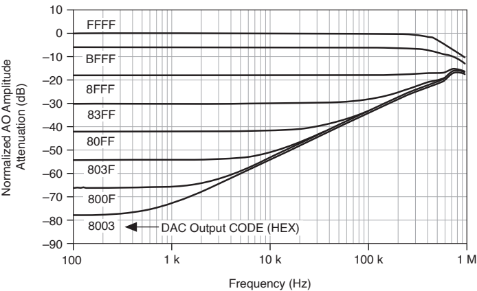
Figure 7. AO <0..3> External Reference Bandwidth
