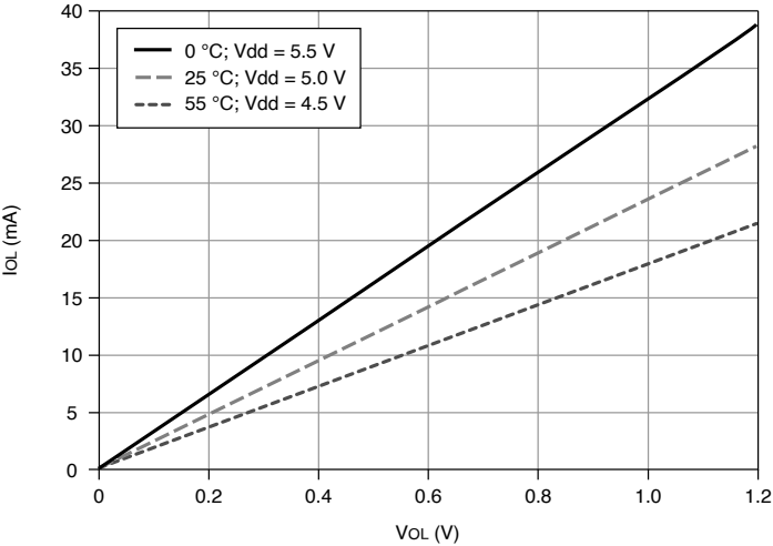
Figure 11. PFI <0..15>/P1/P2: I OL versus V OL
