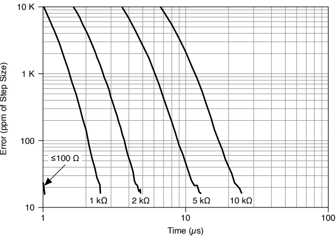
Figure 6. Settling Error versus Time for Different Source Impedances
