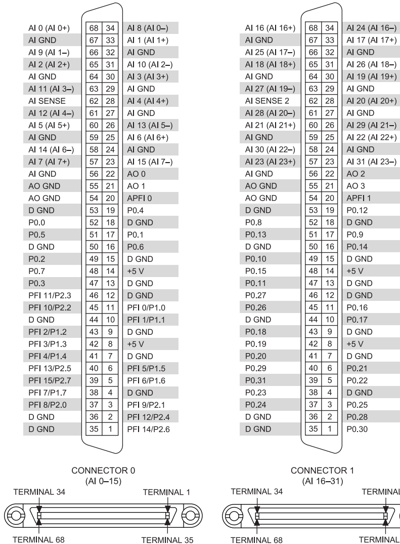
Figure 1. USB-6363 Mass termination Pinout
