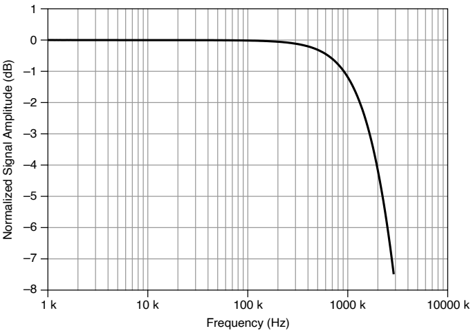
Figure 5. AI <0..31> Small Signal Bandwidth
