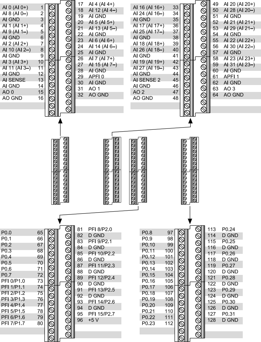
Figure 2. USB-6363 Screw Terminal Pinout
