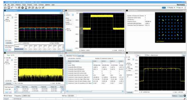
Constellation, Summary View, CHP, and SEM displays supported in option 5G NR
