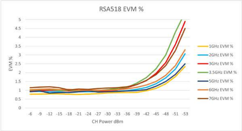
For RSA518 Series Spectrum Analyzers: \leq 39.2 dB rms EVM from 1 GHz to 7 GHz
