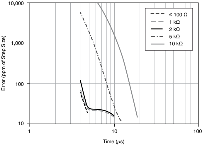
Figure 2. Settling Error versus Time for Different Source Impedances
