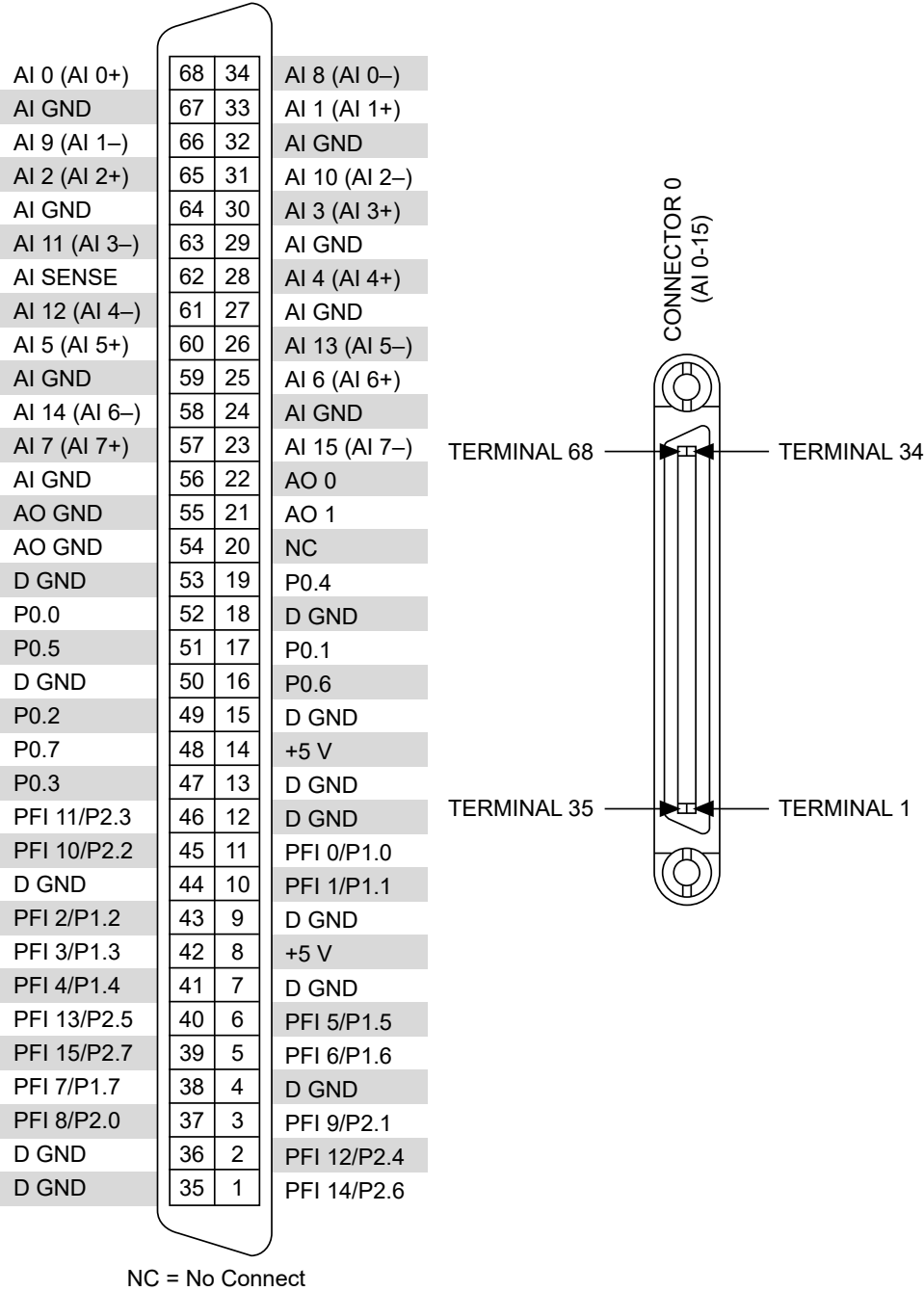
Figure 1. PCIe-6321 Pinout
