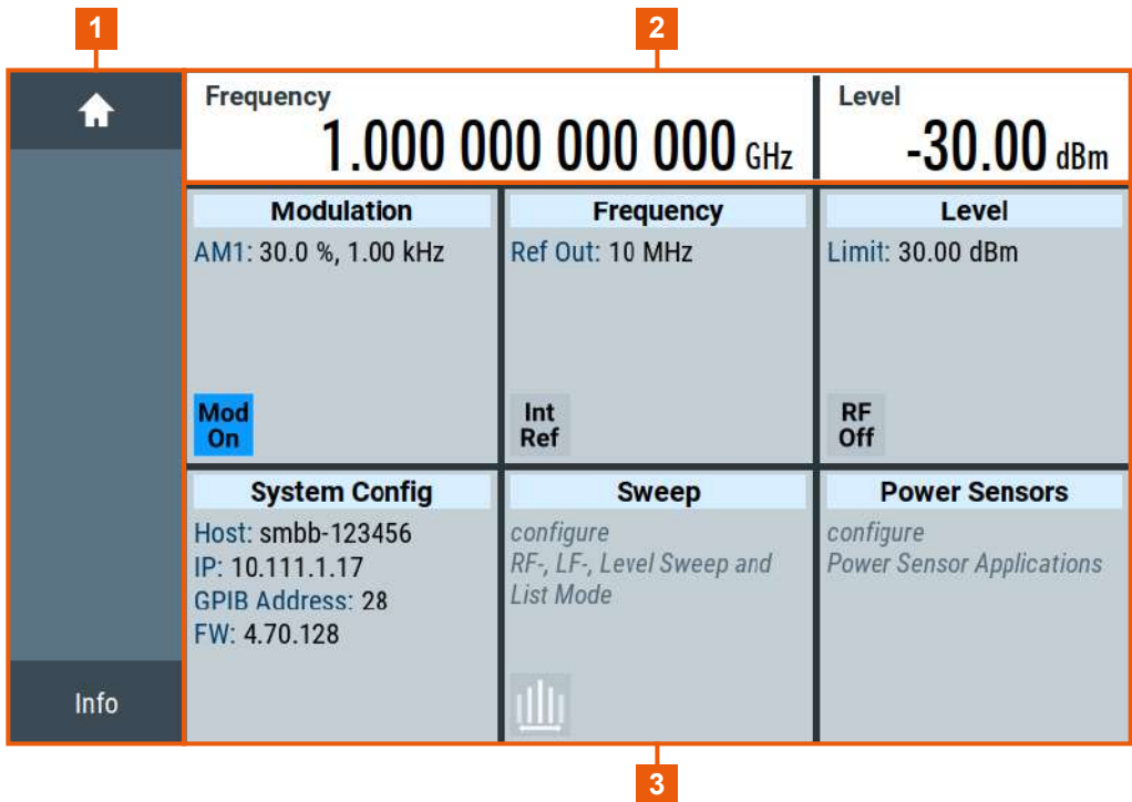
Figure 7-1: Home screen
