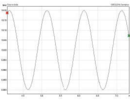
Figure 4: 10 MHz with 1kHz FM - Modulation domain view.
