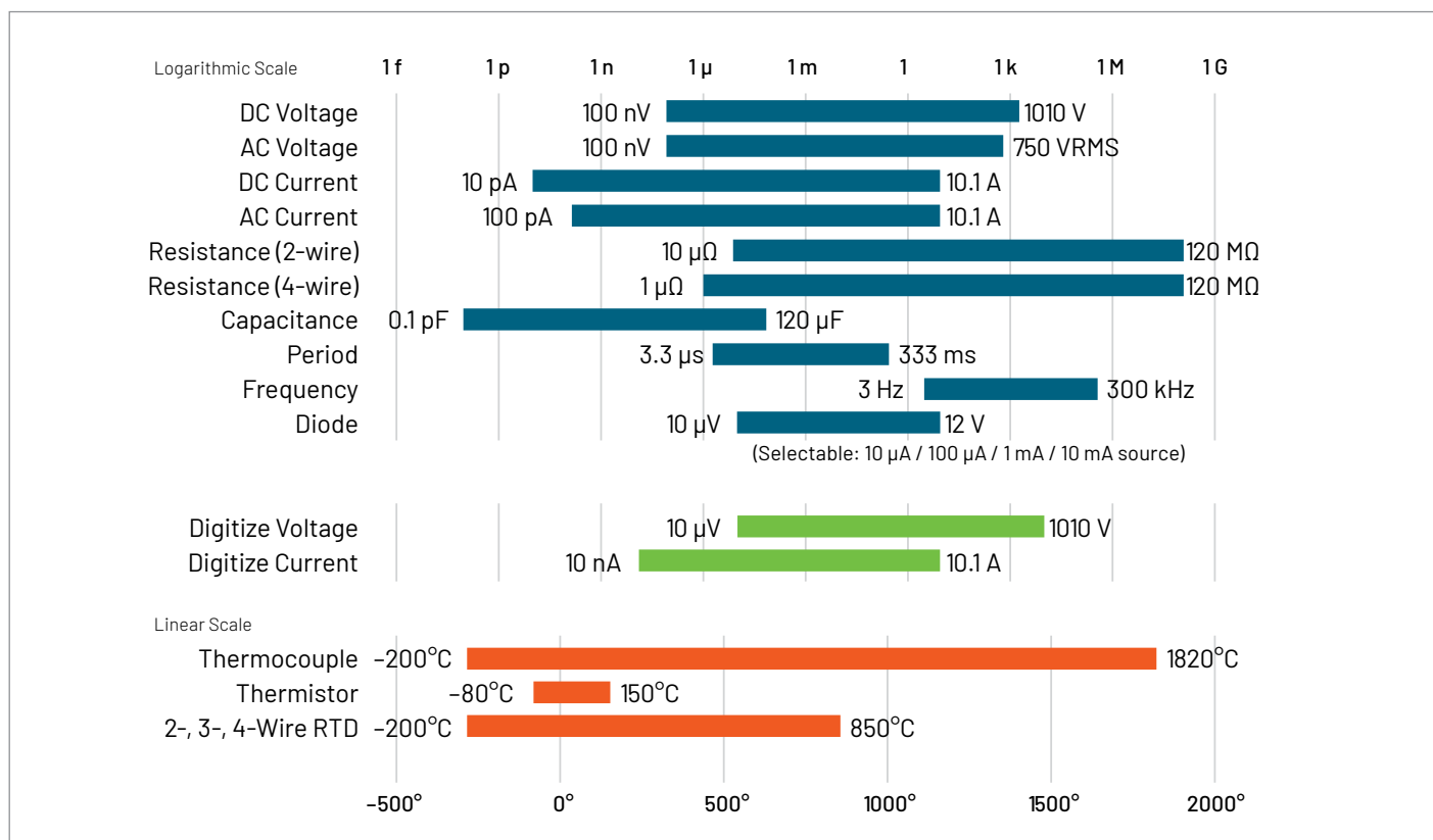
DMM6500 15 measurement functions and ranges.
