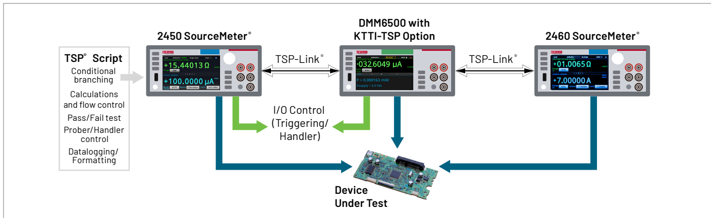
TSP System using TSP-Link for instrument to instrument communication.
