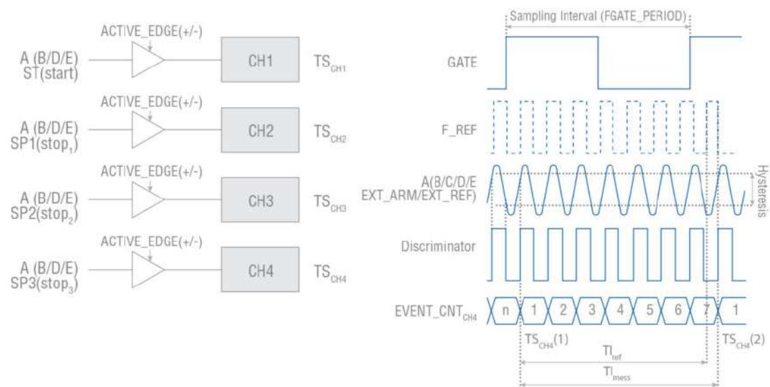
Fig. 5.14: TIE measurement
