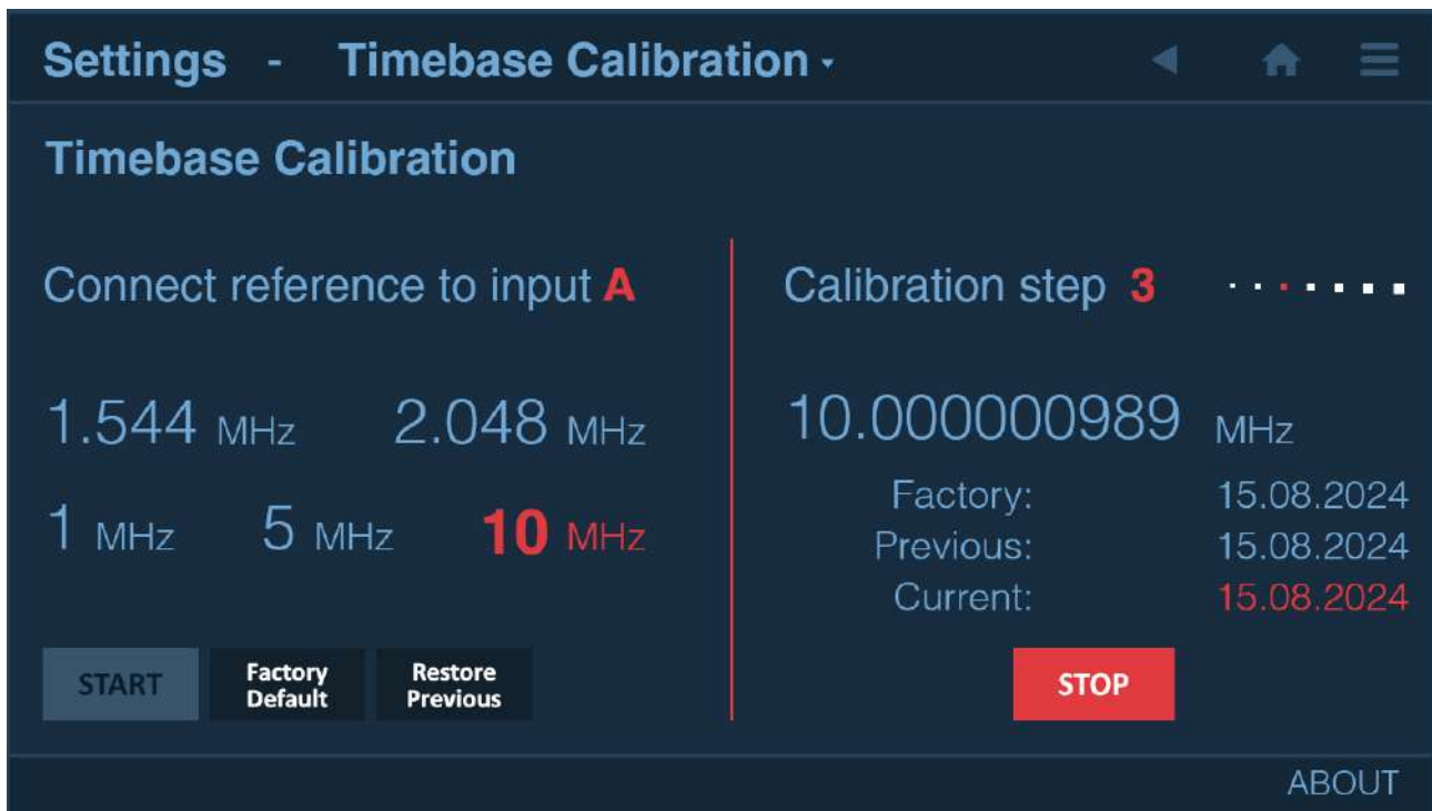
Fig. 7.7: Timebase Calibration menu
