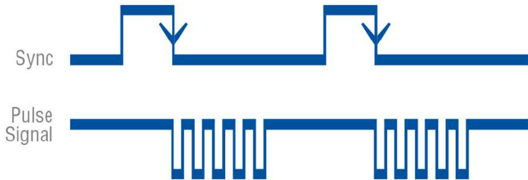
Fig. 4.21: Sync signal used as start arming starts the measurement.
