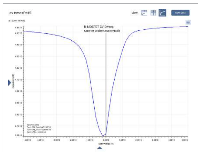
Capacitance-Voltage sweeps.
